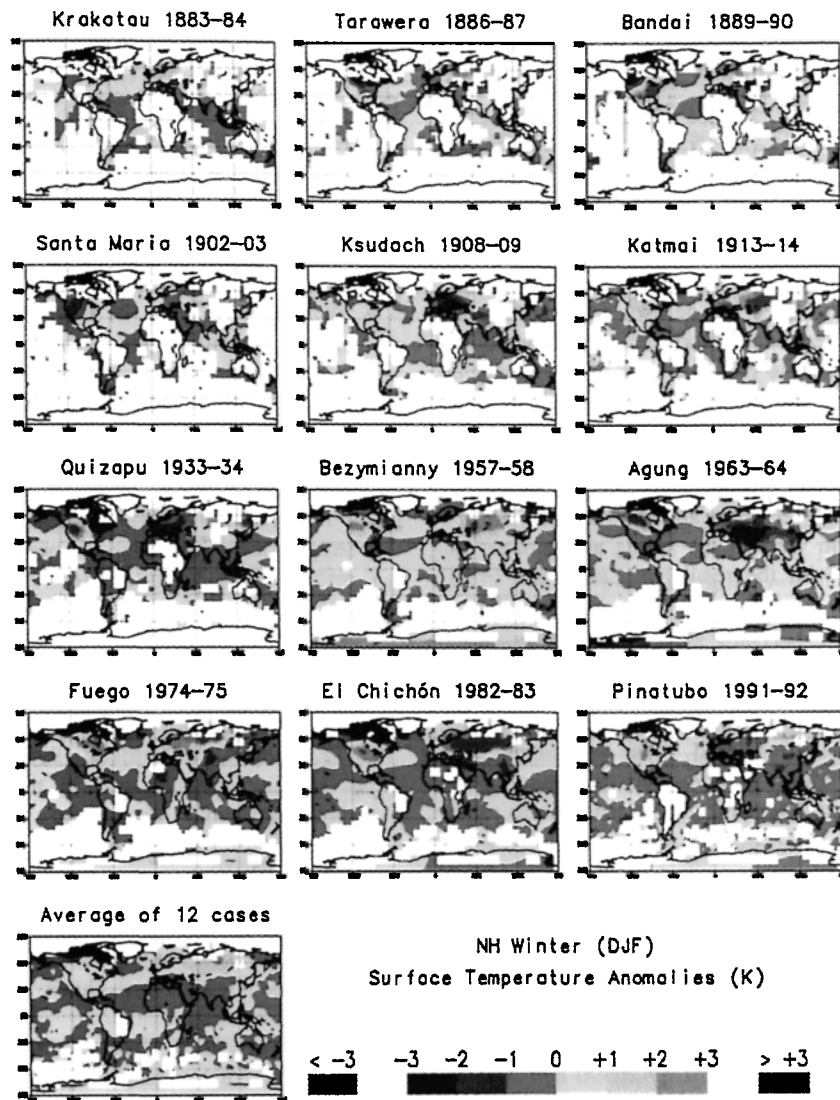
Fig. 1. Northern Hemisphere winter (DJF) surface temperature anomalies for the indicated years (the winter following the tropical volcanic eruptions, the first or second winter following the midlatitude eruptions, and two winters following the high-latitude ones), and the average of the 12 cases.
