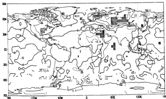
Fig. 2. Average of the 12 winter surface temperature anomalies shown in Fig. 1 (same as last map in Fig. 1, but with contour interval = 0.5°C), with shading indicating the regions for which this average is significantly different from the average of the winters for all the other years between 1866 and 1992 at the 95% level according to a Student's t-test.
