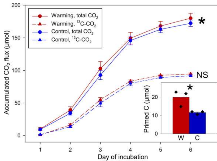
Fig. 2 The accumulated CO 2 flux and the priming effect during the 6-day incubation trial. Red lines/symbols represent in situ warmed soils (W) and blue lines/symbols represent unwarmed/control soils (C). Solid lines represent total CO 2 and dashed lines represent 13 C-CO 2 . The significance of the difference was determined by one-way ANOVA ( n = 3 , biological replicates of warmed or control samples) on CO 2 amounts and primed C amounts between warmed and control samples (shown in the inset of the figure). W, warmed samples; C, control samples; NS, not significant. Data are shown as mean \pm standard error
