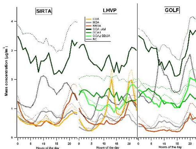
Fig. 8. Diurnal patterns of the PMF factors (solid line = median values, dashed line = mean values). For comparison, the OOA total, which represents the sum of OOA 1 and OOA 2 -BBOA when these two sources were identified separately by PMF, is shown.
