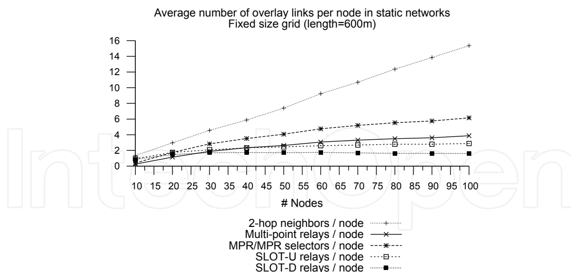
Fig. 12. Density of MPR and SLOT overlays in static networks. The SLOT-D simulations are computed with the quantized cost: cost(\overline{xy}) = \lceil K \frac{d(\overline{xy})}{r} \rceil , with K = 10 and d(\overline{xy}) being the Euclidean distance between x and y .
