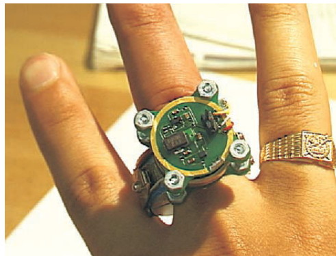
Fig. 1. Photograph of PPG Ring Biosensor Prototype (Courtesy of Asada et. al [2])
