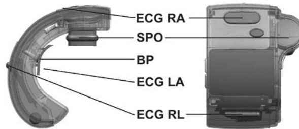
Fig. 2. Photograph of AMON Sensors: ECG, SPO 2 , and Blood Pressure (Courtesy of Anliker et. al [7])
