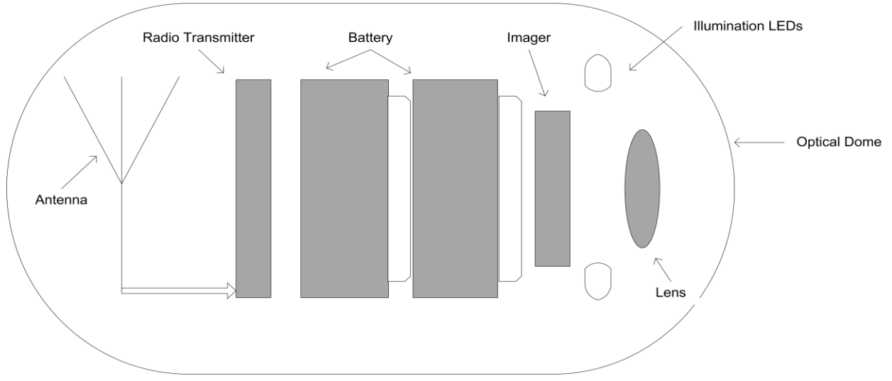
4 Fig. 1. Capsule endoscopy [6]
