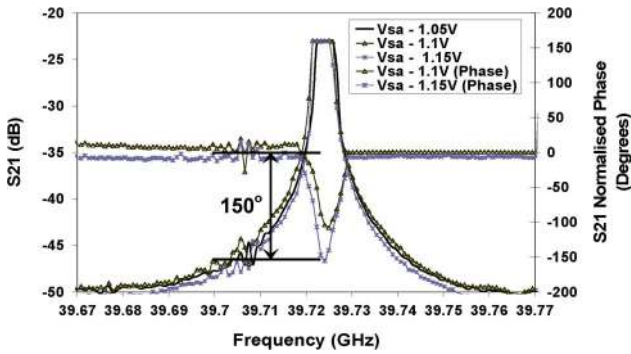
Fig. 11. Measured magnitude and phase of S_{21} at different SA reverse bias values (Phases are normalized to V_{sa} = -1.05 V) for MLL-A2, Distance between horn and patch Antennas = 20 cm.
