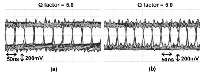
Fig. 16. Downconverted NRZ data eye diagrams for the data rates of (a) 20 Mb/s NRZ data eye diagram and (b) 22 Mb/s NRZ data eye diagram using horn to patch antenna and MLL for BPSK data transmission using wireless injection locking technique, distance between antennas = 10 cm.
