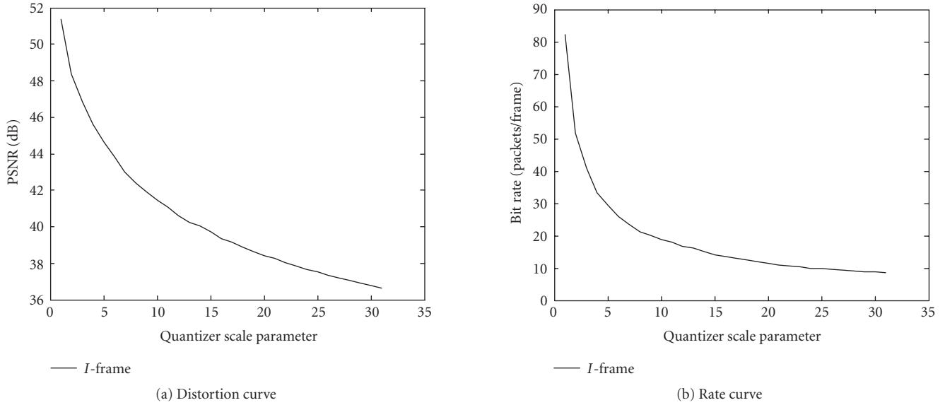
FIGURE 5: Rate-distortion curves.
