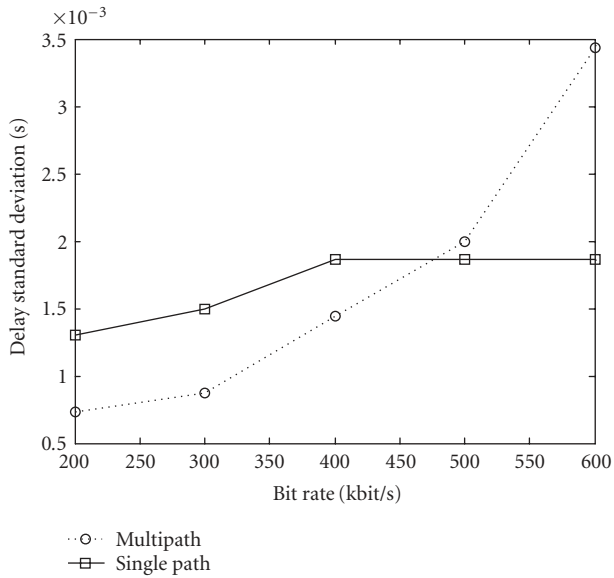
FIGURE 9: End-to-end delay standard deviation.
