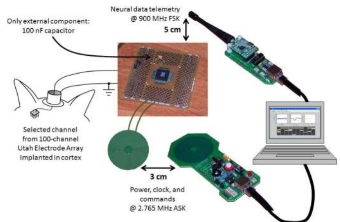
Fig. 8. Wireless testing configuration for in vivo experiments using INI3 chip with one external capacitor. Power and commands are delivered wirelessly via inductive link; telemetry is received via 900 MHz antenna.
