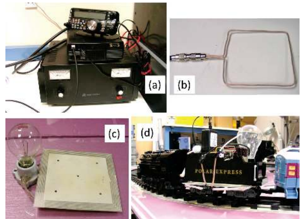
Fig. 11. Components of WPT experiment with array of resonators: (a) RF power transmitter; (b) square antenna to inductively couple power from the RF transmitter to the system; (c) a wireless power receiver composed of a resonant coil, a loop antenna and a 40W light bulb; (d) a wireless power receiver with a resonant coil and a loop antenna to pick up RF power, a rectifier and regulator to convert RF power to DC, and a motor for the toy train set and a 40W light bulb as load.
