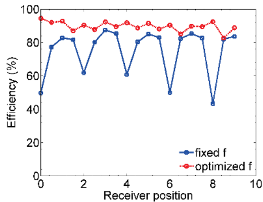
Fig. 9. Power transfer efficiency for one receiver as functions of receiver position in unit of lattice size of the array, operating at a fixed frequency and optimized frequency for each position.
