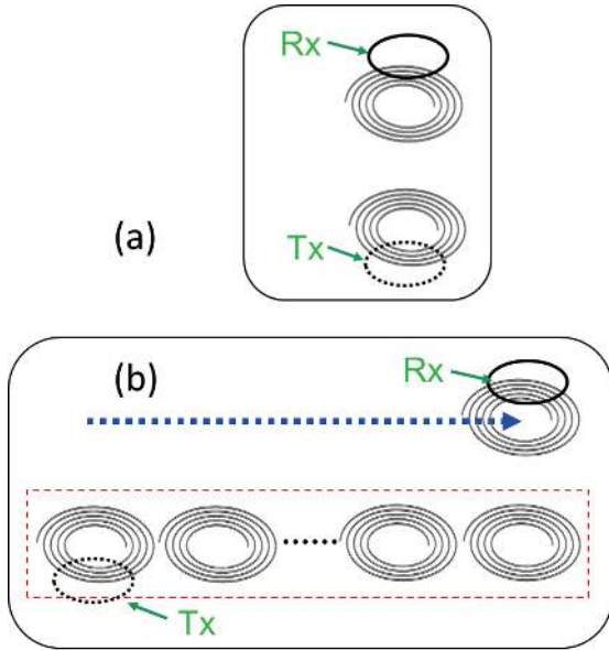
Fig. 5. (a) WPT system with one resonant coil as transmitter and one resonant coil as receiver. (b) WPT system with an array of resonant coils as transmitter and one resonant coil as receiver.
