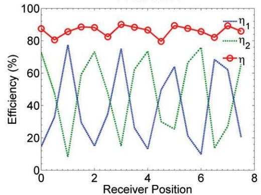
Fig. 8. Power transfer efficiency for two individual receivers and the combined efficiency, as functions of receiver position in unit of lattice size of the array. Operating frequency is fixed.
