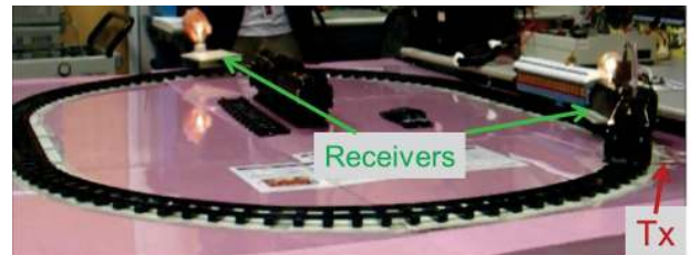
Fig. 11. Components of WPT experiment with array of resonators: (a) RF power transmitter; (b) square antenna to inductively couple power from the RF transmitter to the system; (c) a wireless power receiver composed of a resonant coil, a loop antenna and a 40W light bulb; (d) a wireless power receiver with a resonant coil and a loop antenna to pick up RF power, a rectifier and regulator to convert RF power to DC, and a motor for the toy train set and a 40W light bulb as load.
