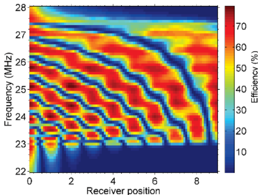
Fig. 7. Power transfer efficiency from a 10-resonator array to a resonant receiver, as functions of receiver position in unit of lattice size of the array.
