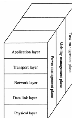
Fig. 3 Protocol Stack of WSN [2]
