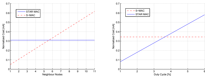
(a) Normalized Cost vs. Neighbor Nodes (b) Normalized Cost vs. Duty Cycle Duration
