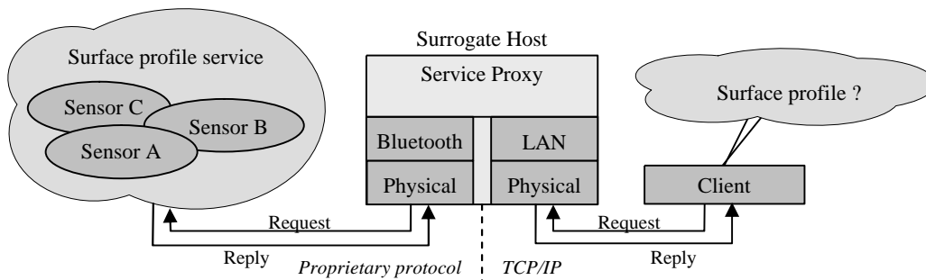
Fig.3 Example of a Surrogate Architecture in Sensor Networks
