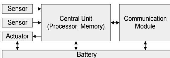
Fig.1 Structure of a Sensor Node
