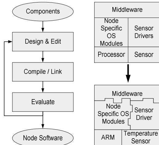
Fig.5 a) Development Process of Node Software, b) Example of a Node Software with Optimized Interfaces
