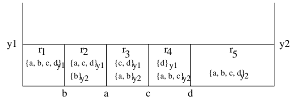
Figure 6: Regions and labels of regions.
