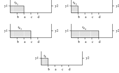
Figure 7: Region intersection for node z of N' .
