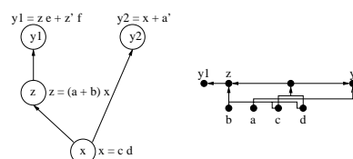
Figure 2: Network N' and its optimal placement.
