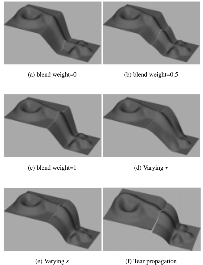
Figure 18: Control over stitch parameters.
