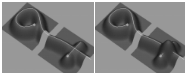
Figure 10: Multiple wires on multiple surfaces with differing deformations. Left, (a): integrated deformation that avoids blobby superposition. Right, (b): the traditional additive deformation.
