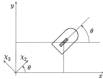
Fig. 2. Relevant variables for the unicycle (top view).
