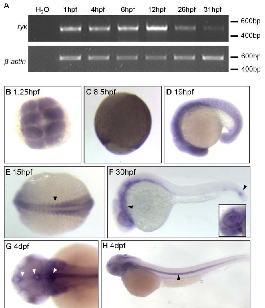
Figure 1. Zebrafish ryk expression profile. (A) Semiquantitative RT-PCR showing temporal ryk expression. (B–E) Whole-mount in situ hybridization reveals ubiquitous ryk expression throughout maternal (B) and gastrula stages (C–E) with enrichment in somites (E, arrowhead) and the central nervous system. (F) At 30 hpf, ryk is expressed in the brain and tail (arrowheads) and notably the eyes (inset). (G and H) At 4 dpf, ryk is expressed in the lining of ventricular zones (G, arrowheads) and notochord (H, arrowhead). Stages and orientation: 1.25 hpf, animal pole view; 8.5 hpf, lateral view; 15 hpf, dorsal view with anterior to the left; 19 and 30 hpf, lateral view with anterior to the left; 4 dpf, dorsal view of brain and lateral view of the whole body, anterior to the left.
