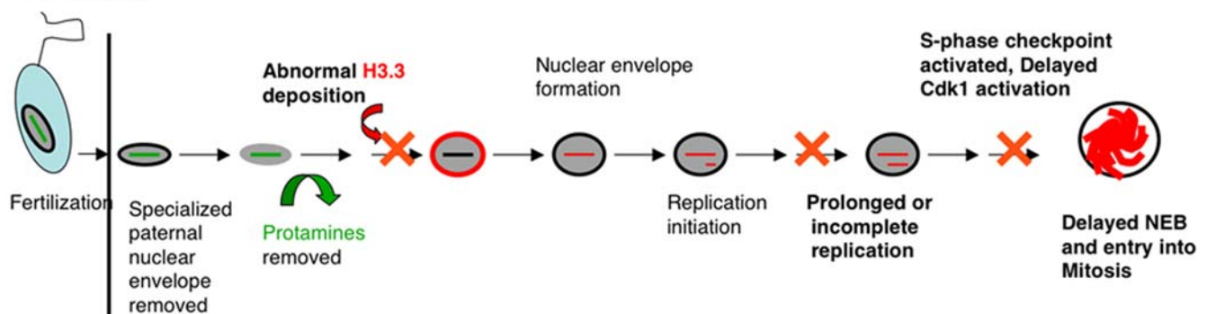
Figure 5. A schematic of key events in the transformation of sperm to male pronucleus in embryos from normal and CI crosses. Normal cross: Immediately following fertilization, the specialized nuclear envelope (lacking nuclear pores) of the male pronucleus is removed. Next, the protamines are removed and replaced by maternally supplied histones, including the replication-independent histone H3.3. This event is followed by lamin deposition and formation of a conventional nuclear envelope containing nuclear pores. Next, S-phase is initiated and upon completion, Cdk1 is activated driving nuclear envelope breakdown, chromosome condensation, and spindle assembly. CI cross: At the cytological level, removal of the sperm nuclear envelope and protamines appear normal. Often however, histone H3.3 deposition is abnormal, resulting in a ring of histone H3.3 encompassing the paternal pronucleus. This is the earliest documented CI phenotype in embryos and is similar to that observed for mutants in the chromatin remodeling protein Chd1. Imaging PCNA, a marker for replicating chromosomes, indicates that replication initiates normally in CI embryos, but is prolonged or incomplete. This may be a direct result of the earlier defects in H3.3 deposition. Replication delays activate S-phase checkpoints and thus are likely the cause of the previously described delays in Cdk1 activation and nuclear envelope breakdown. doi:10.1371/journal.ppat.1000343.g005
