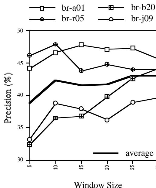
Figure 5: context size and different files
