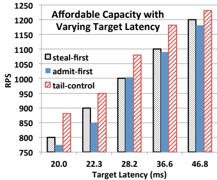
Figure 12: The Bing workload results. Tail-control increases system capacity for different target latencies. Tail-control compared to steal-first and admit-first.
