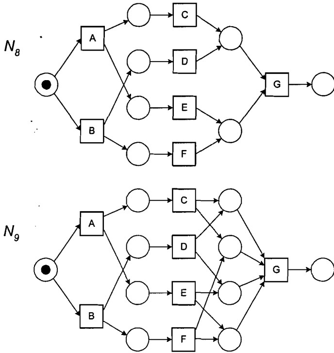
Fig. 7. WF-net N_8 cannot be rediscovered. Nevertheless \alpha returns a WF-net which is behavioral equivalent.
