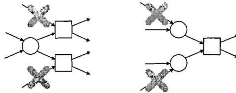
Fig. 3. Two constructs not allowed in SWF-nets.
