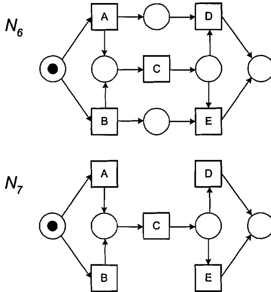
Fig. 6. The non-free-choice WF-net N_6 cannot be rediscovered.
