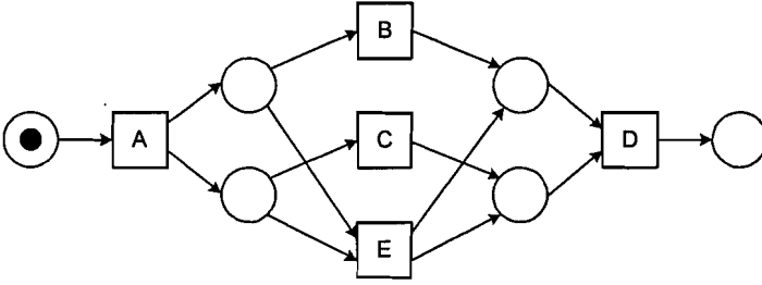
Fig. 5. Another process model corresponding to the workflow log shown in Table 1.
