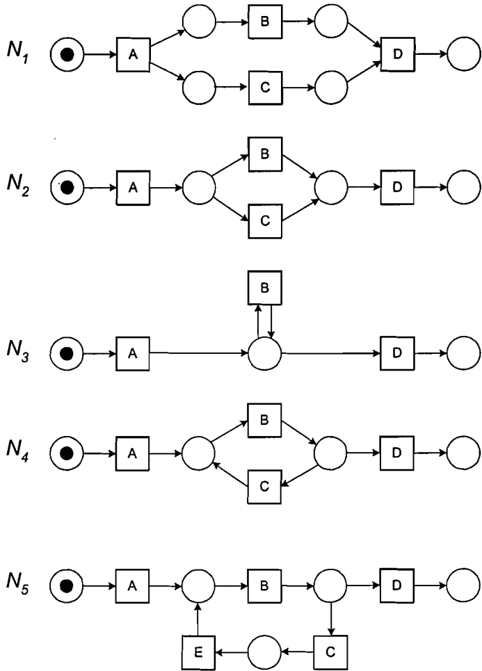
Fig. 4. Five sound SWF-nets.
