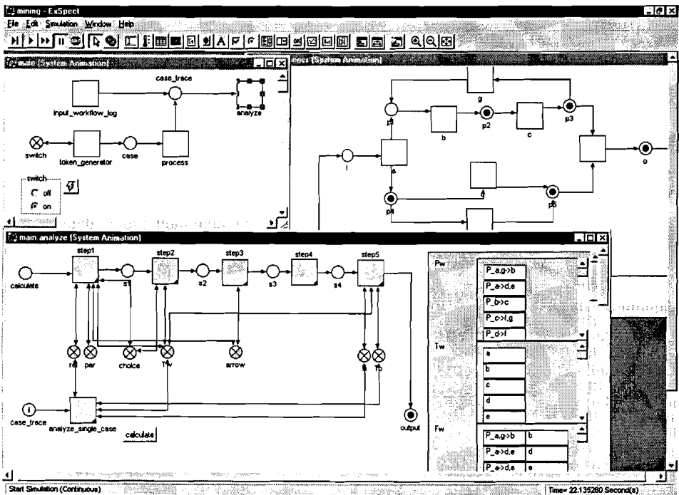
Fig. 8. A screenshot of the ExSpec module MiMo while mining a workflow process.
