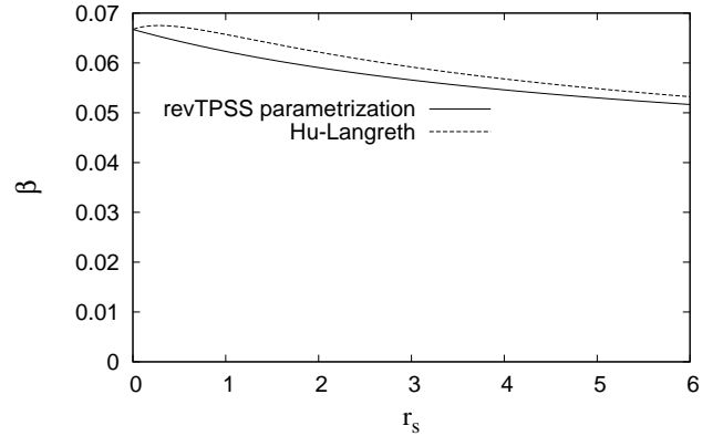
FIG. 3: Finite-range contribution to the gradient coefficient for correlation, as a function of density parameter r_s , from Ref. [22] and from Eq. (3).
