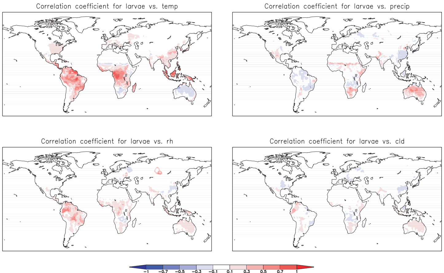
Fig. 2. Linear correlation coefficients between modelled mosquito ( Aedes aegypti ) larvae and CRU05 climate data, based on monthly anomalies (deviations from the long-term mean), for 1958 to 1995. Correlation coefficients between larval anomalies and (a) temperature anomalies, (b) precipitation anomalies, (c) relative humidity anomalies, (d) cloud cover anomalies
