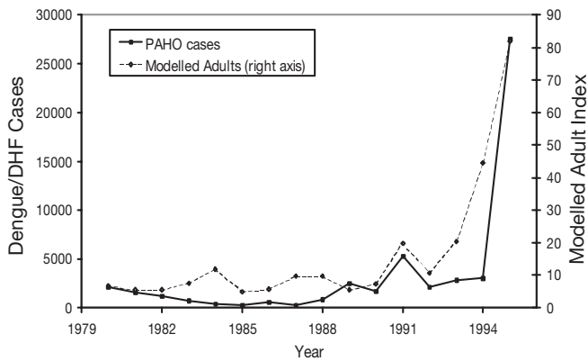
Fig. 5. Honduras: Dengue/DHF cases (PAHO dataset) and modelled adult mosquito ( Aedes aegypti ) index. Correlation coefficient = 0.91* (0.88* detrended); *p < 0.05
