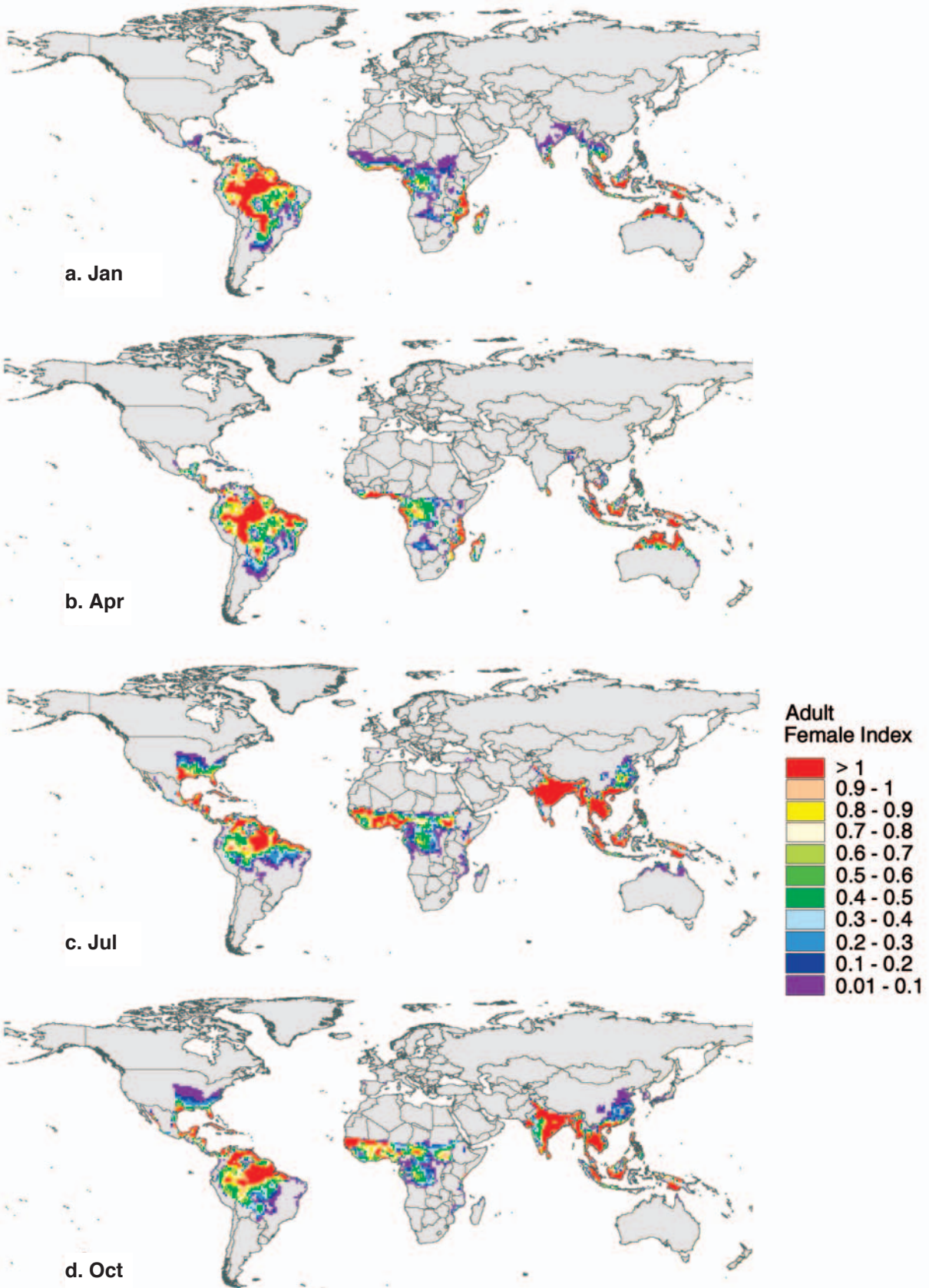
Fig. 1. Modelled potential adult female mosquito Aedes aegypti index (mosquitos m^{-2} of container surface water), for (a) January, (b) April, (c) July, (d) October
