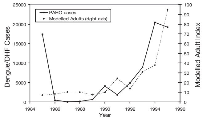
Fig. 6. Nicaragua: Dengue/DHF cases (PAHO dataset) and modelled adult mosquito ( Aedes aegypti ) index. Correlation coefficient = 0.64* (0.49 detrended); *p < 0.05
