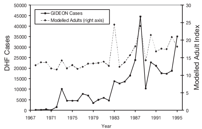
Fig. 4. Indonesia: DHF cases (GIDEON dataset) and modelled adult mosquito ( Aedes aegypti ) index. Correlation coefficient = 0.77* (0.58* detrended); * p < 0.05
