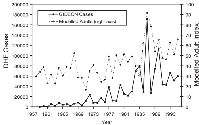
Fig. 3. Thailand: DHF cases (GIDEON dataset) and modelled adult mosquito ( Aedes aegypti ) index. Correlation coefficient = 0.68* (0.43* detrended); * p < 0.05
