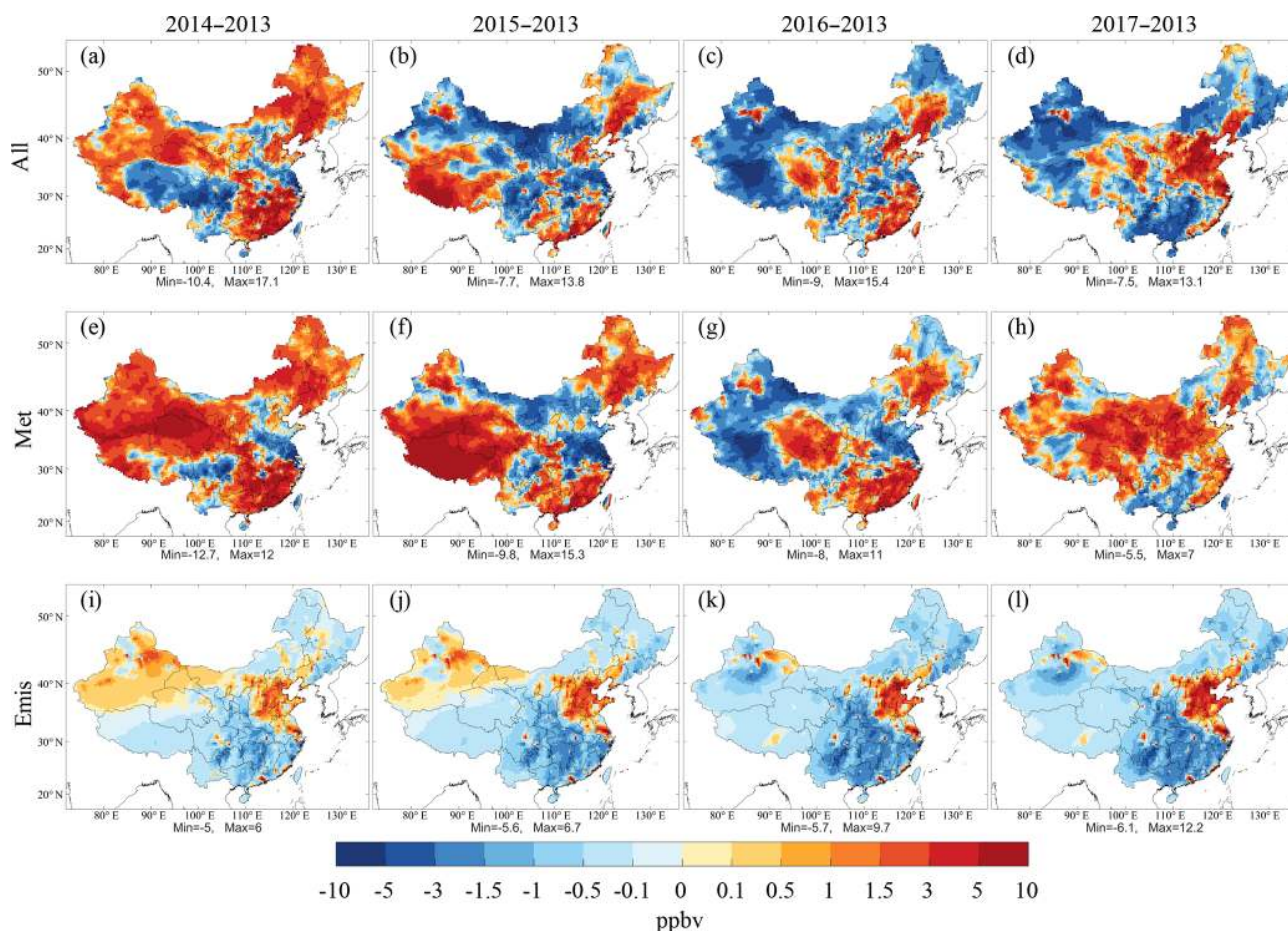
Figure 3. Changes in the simulated summer surface MDA8 O 3 mixing ratios from the base simulation (All, a–d); those due to variations in meteorological conditions (Met, e–h); and anthropogenic emissions (Emis, i–l) in 2014, 2015, 2016, and 2017 relative to 2013.
