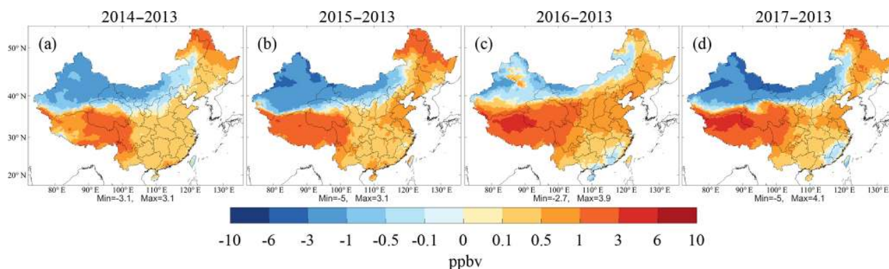
Figure 7. Changes in the simulated summer surface MDA8 O 3 mixing ratios due to variations in long-range transport in 2014, 2015, 2016, and 2017 relative to 2013.
