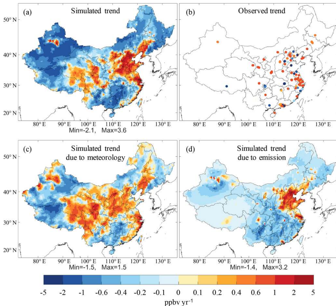
Figure 2. Rates of changes in the simulated (a) and observed (b) surface MDA8 O 3 mixing ratios in summer from 2013 to 2017. In panel (b), only environmental monitoring sites (493) with data available in all 5 years are presented. (c) and (d) present the rates of changes in the simulated MDA8 O 3 mixing ratios due to variations in meteorological conditions and anthropogenic emissions in summer from 2013 to 2017 (see Methods section). The corresponding p values of regression are presented in Fig. S2.
