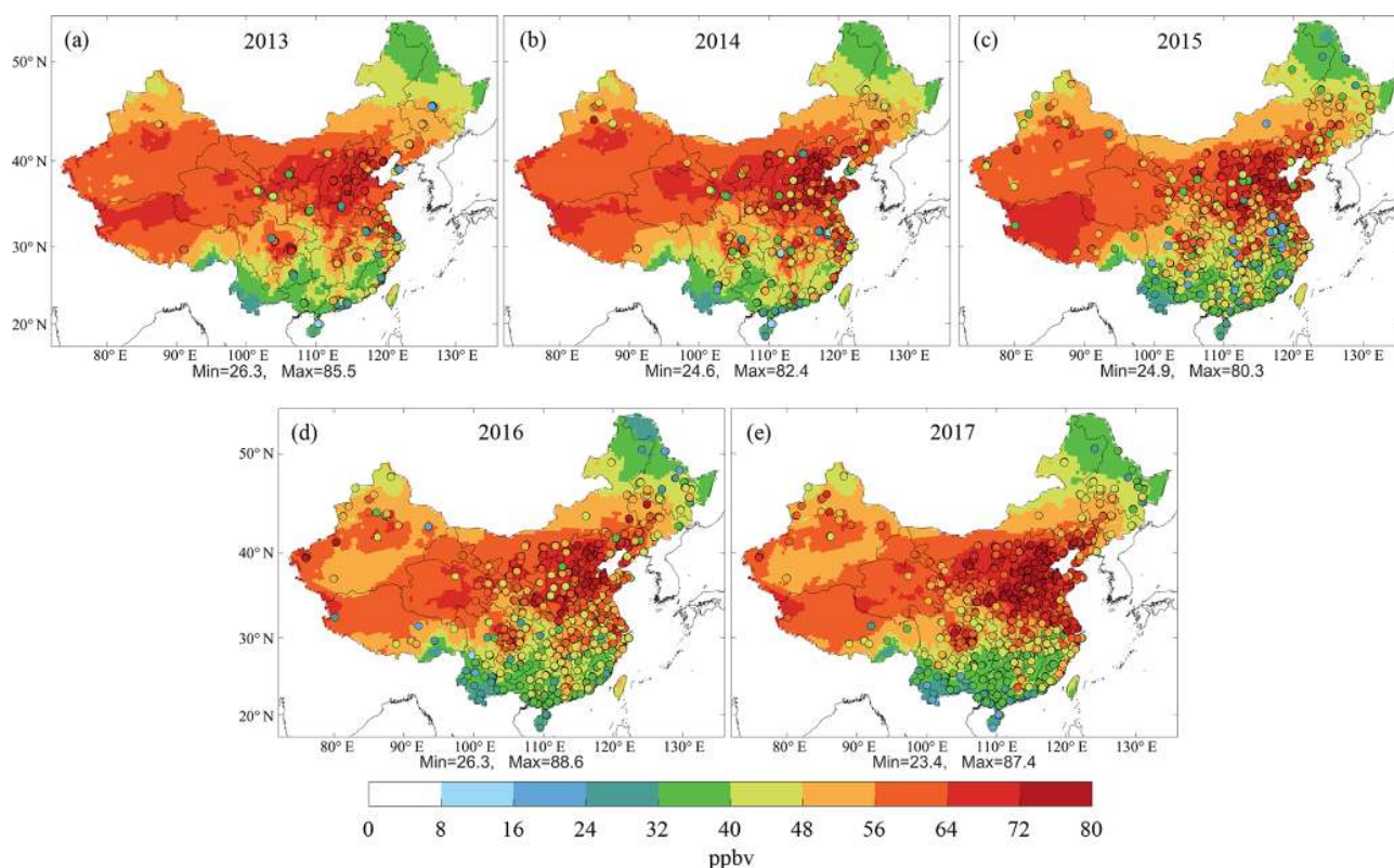
Figure 1. Spatial distribution of the simulated surface maximum daily 8 h average (MDA8) \text{O}_3 mixing ratios in summer (June–August) of 2013 (a), 2014 (b), 2015 (c), 2016 (d), and 2017 (e). Circles with color are the available observed values at environmental monitoring stations in each year.
