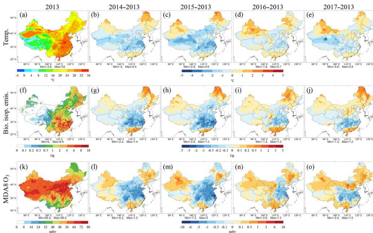
Figure 5. The simulated daytime averaged temperature at a height of 2 m (Temp., a–e) and total biogenic isoprene emissions (Bio. isop. emis., f–j) in summer of 2013 from the base simulations and their changes in 2014, 2015, 2016, and 2017 relative to 2013. Panels (k)–(o) (MDA8 O 3 ) show the simulated summer surface MDA8 O 3 mixing ratios in 2013 from the base simulation and their changes due to variations in biogenic emissions in 2014, 2015, 2016, and 2017 relative to 2013.
