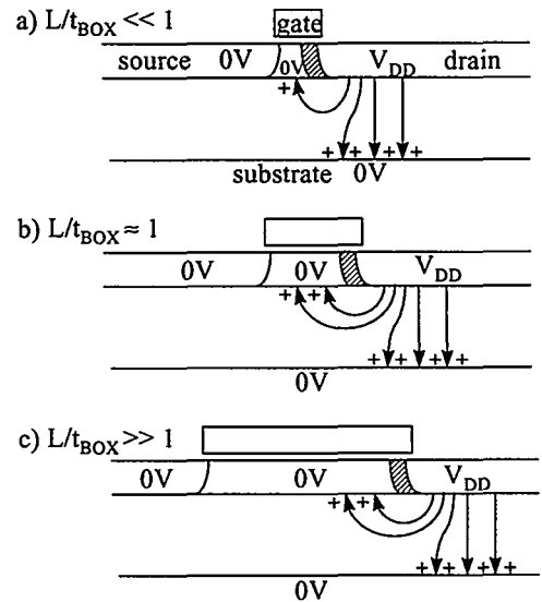
Fig. 7. Schematic representation of field lines and hole trapping in the buried oxide of NMOS/SOI transistors with varying L/t BOX ratio. The grounded body transistors are OFF biased during irradiation.
