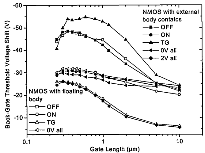
Fig. 3. Back-gate threshold voltage shift versus gate length of NMOS/SOI UNIBOND transistors measured on the Id-Vb characteristics at drain voltage of V_{\text{d}}=0.1\text{V} at a dose of 1Mrad( \text{SiO}_2 ).
