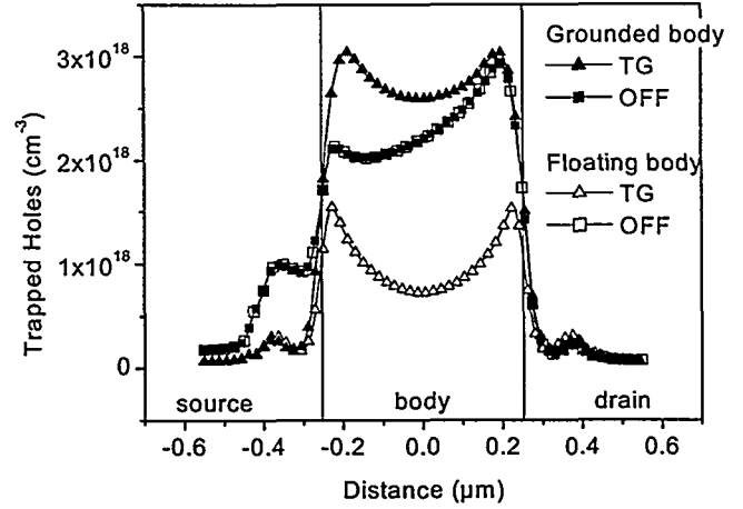
Fig. 6. Simulated trapped hole profiles in the buried oxide, 6 nm under the front interface, for TG and OFF cases, at 1 Mrad(SiO 2 ). The simulated transistor is either a floating or grounded body NMOS with a gate length of 0.5 \mu m.
