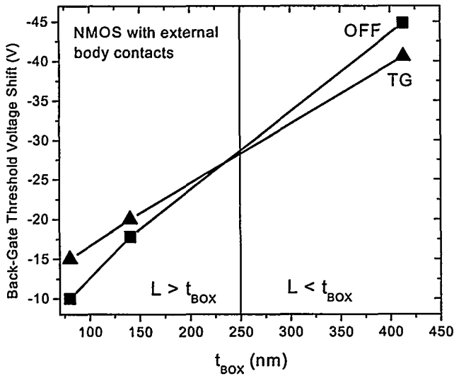
Fig. 4. Back-gate threshold voltage shift versus buried oxide thickness of 0.25 \mu m gate length NMOS/SOI transistors measured on the Id-Vb characteristics at a drain voltage of Vd=0.1V and at a dose of 1Mrad(SiO 2 ).
