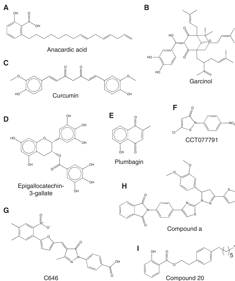
Figure 5. HAT inhibitors. Reported inhibitor specificities are as follows: (A,B,F) specific to p300 and PCAF; (C–E) specific to p300; (G) specific to p300; (H,I) specific to MYST.
