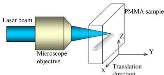
Fig.1 Schematic of transverse direct writing by fs laser. The laser beam propagates in the y-direction, with the sample translated in the x-direction
