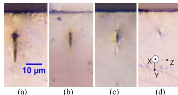
Fig.6 Optical microscope images of the cross-sectional shape of inscribed structures. The incident energies E_p were (a) 250 nJ, (b) 200 nJ, (c) 100 nJ and (d) 70 nJ, with v_s=1 \text{ mm/s} .
