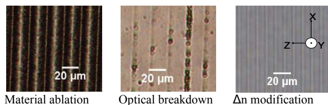
Fig.3 Microscope images of three stages of microstructure outcomes (top view)
