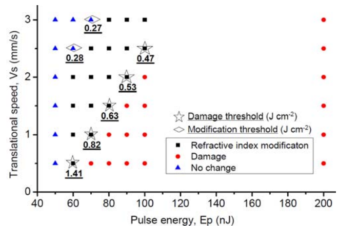
Fig.5 Damage and modification produced by varying v_s and E_p at a constant F_d=100 \mu\text{m} .
