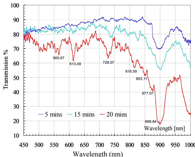
Fig.10 Change in transmission of a 250µm period LPG as a function of time.
