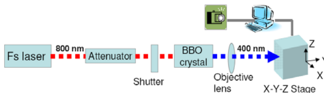
Fig.2 Schematic of experimental system
