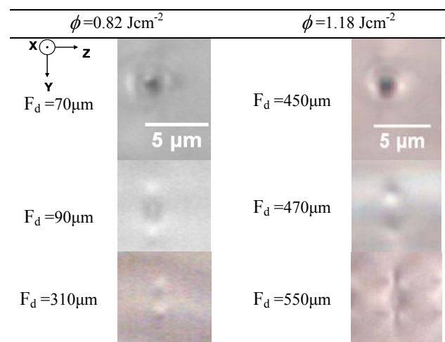
Fig.8 Cross section view of outcomes of laser irradiation with fluence of 0.82\text{Jcm}^{-2} ( E_p=70\text{nJ} , v_s=1\text{mm/s} ) and 1.18\text{Jcm}^{-2} ( E_p=100\text{nJ} , v_s=1\text{mm/s} ) at different focusing depths ( F_d ).
