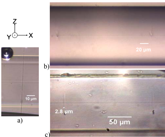
Fig.9 A section of LPG demonstrates (a) the continuous inner structural change induced by fs lasers within the sandwich setup. A part of in-fibre grating is shown in (b) cross view and (c) side view.
