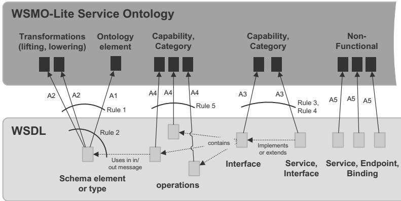
Fig. 2. Illustration of Annotations and Rules
