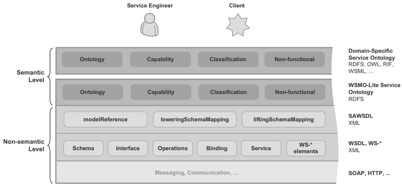
Fig. 1. Semantic Service Stack
