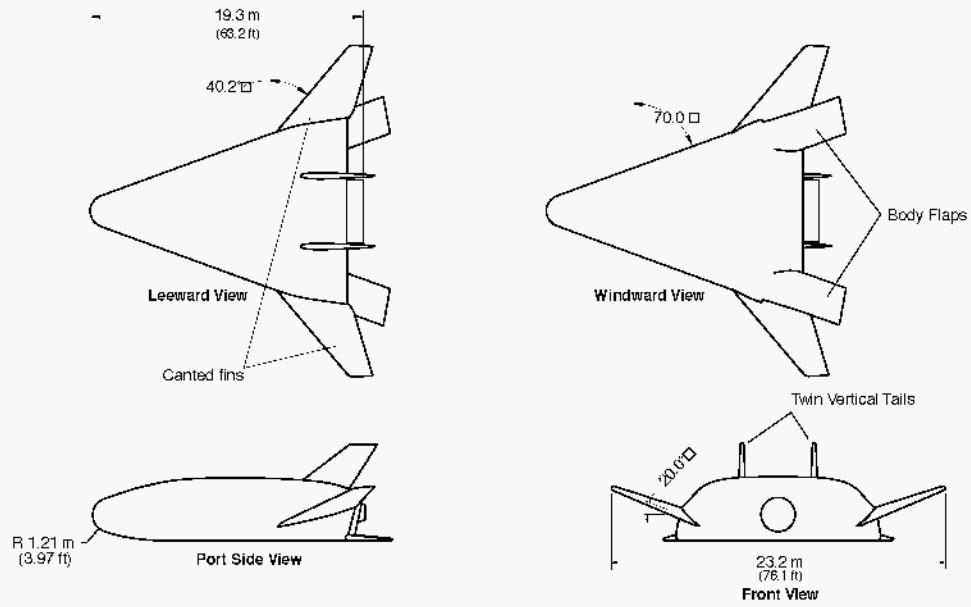
Figure 1. Sketch of Full-Scale X-33 604B00021EG Configuration
