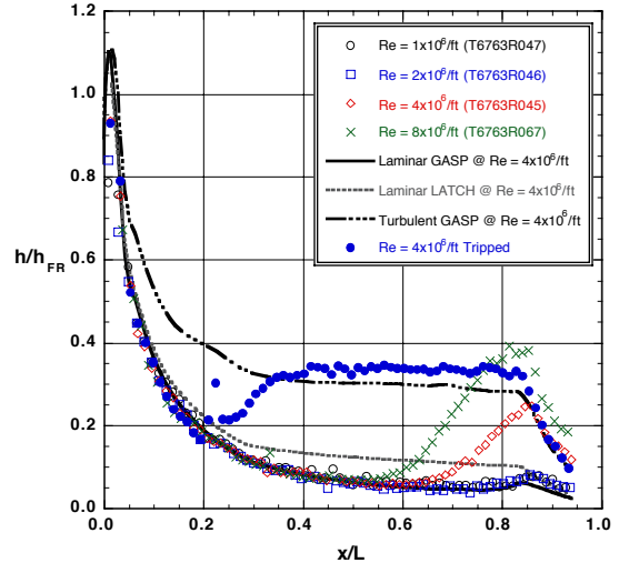
Fig 10b Effect of Re for smooth and tripped cases at \alpha = 30 -deg as compared to prediction
