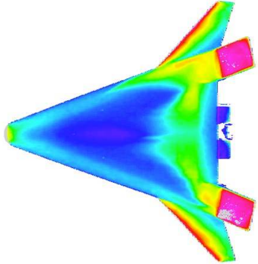
Fig 9b Effect of \alpha on smooth body transition patterns for \alpha = 30 -deg, Re = 7.9 \times 10^6/\text{ft} , \delta_{RF} = 20 -deg
