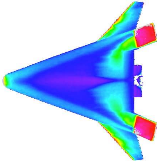
Fig 9a Effect of \alpha on smooth body transition patterns for \alpha = 20 -deg, Re = 7.9 \times 10^6/\text{ft} , \delta_{RF} = 20 -deg
