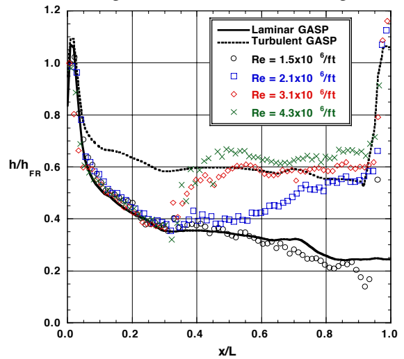
Fig 17b Effect of Re on heating along chine with 0.005-in trips at AL4-40 for \alpha = 40\text{-deg}
