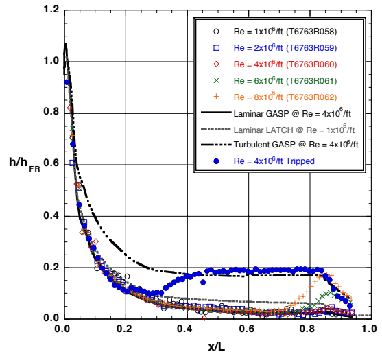
Fig 10a Effect of Re for smooth and tripped cases at \alpha = 20 -deg as compared to prediction
