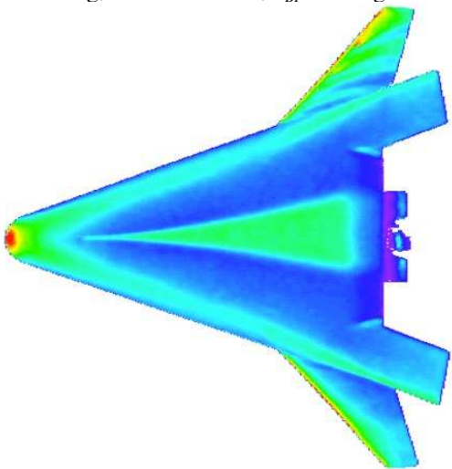
Fig 11c Effect of 0.005-in discrete trip at CL3 for \alpha = 40 -deg, Re = 3.1 \times 10^6/\text{ft} , \delta_{BF} = 0 -deg
