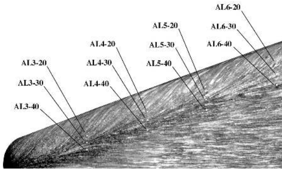
Fig 15 Surface streamlines showing attachment line location for \alpha = 30\text{-deg}
