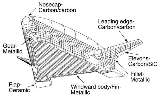
Figure 2 X-33 windward surface TPS.
