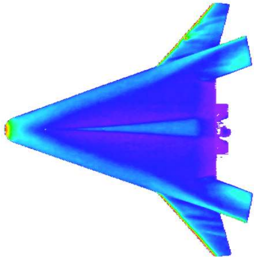
Fig 11a Effect of 0.005-in discrete trip at CL3 for \alpha = 20 -deg, Re = 4.2 \times 10^6/\text{ft} , \delta_{BF} = 0 -deg
