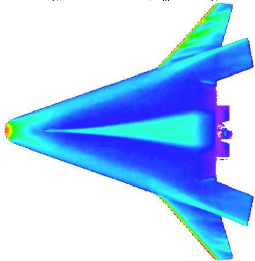
Fig 11b Effect of 0.005-in discrete trip at CL3 for \alpha = 30 -deg, Re = 4.2 \times 10^6/\text{ft} , \delta_{BF} = 0 -deg
