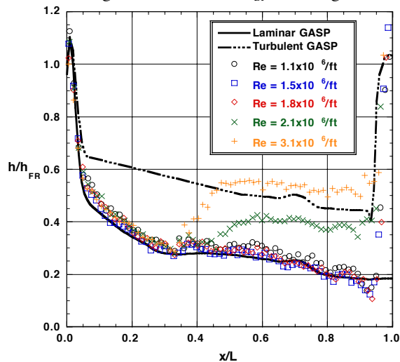
Fig 16b Effect of Re on heating along chine with 0.005-in trips at AL4-30 for \alpha = 30\text{-deg}
