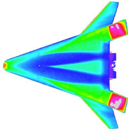
Fig 17a Effect of station-4 0.005-in trips on transition for \alpha = 40\text{-deg} , Re = 3.1 \times 10^6/\text{ft} , \delta_{BF} = 20\text{-deg}
