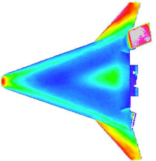
Fig 9c Effect of \alpha on smooth body transition patterns for \alpha = 40 -deg, Re = 7.9 \times 10^6/\text{ft} , \delta_{RF} = 20 -deg
