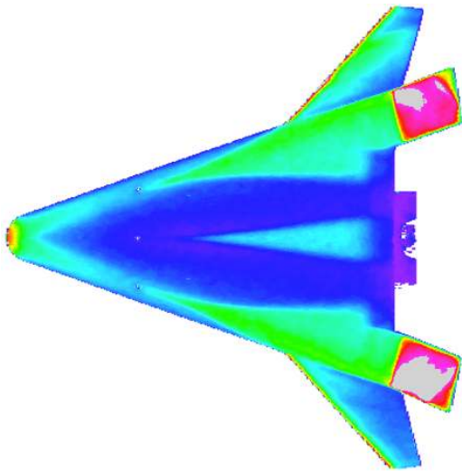
Fig 16a Effect of station-4 0.005-in trips on transition for \alpha = 30\text{-deg} , Re = 3.1 \times 10^6/\text{ft} , \delta_{BF} = 20\text{-deg}
