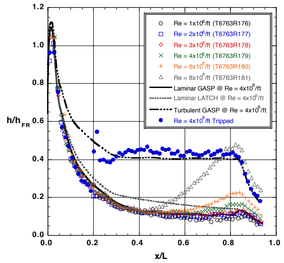
Fig 10c Effect of Re for smooth and tripped cases at \alpha = 40 -deg as compared to prediction
