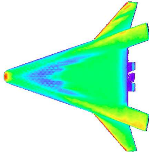
Fig 23 Effect of extended bowed panels ( k=0.008 -in) on heating for \alpha = 40 -deg, Re = 4 \times 10^6 /ft, \delta_{BF} = 0 -deg
