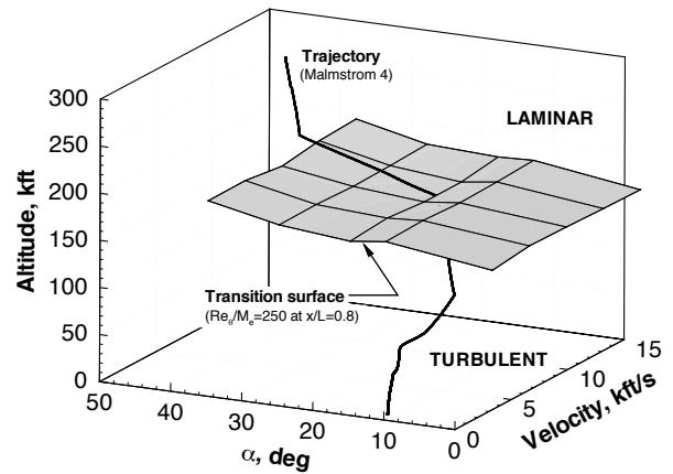
Fig 13 X-33 windward transition criterion based on Re_0/M_e = 250 at x/L = 0.8 on centerline (Ref. 6)
