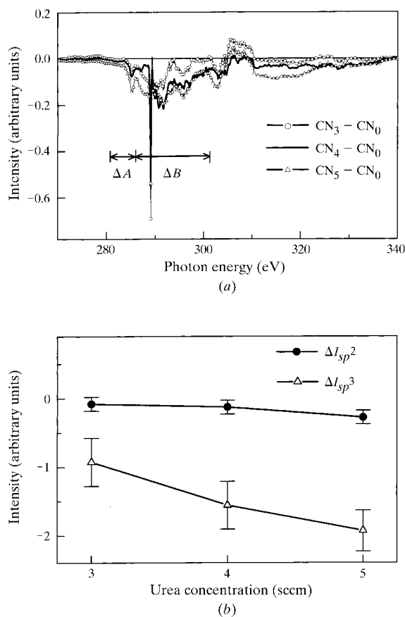
Figure 4 (a) The C K -edge difference intensity curves between N-doped and undoped diamonds. (b) A plot of the integrated difference intensity curves, \Delta I_{sp^2} and \Delta I_{sp^3} , over regions \Delta A(\pi^*) and \Delta B(\sigma^*) , respectively, versus N concentration.
