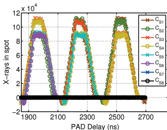
Figure 8 Integrated signal versus the PAD delay with respect to the synchrotron timing with a train imaged by successive in-pixel storage elements. The exposure time was 190 ns and the time between frames was 90 ns. C_{S7} and C_{S8} measured around zero at all PAD delays and are indistinguishable in the figure. Lines are a guide to the eye.
