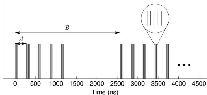
Figure 6 The five trains of bunches as each circulates the synchrotron at CHESS twice. Each individual vertical bar is a bunch of positrons. The trains, from left to right, are referred to as 1–5. Trains 2 and 3 had six bunches and trains 1, 4 and 5 had five bunches. The front-to-front train spacing was 280 ns (labeled A). The revolution period was 2563.2 ns (labeled B). The time between bunches in a train was 14 ns.
