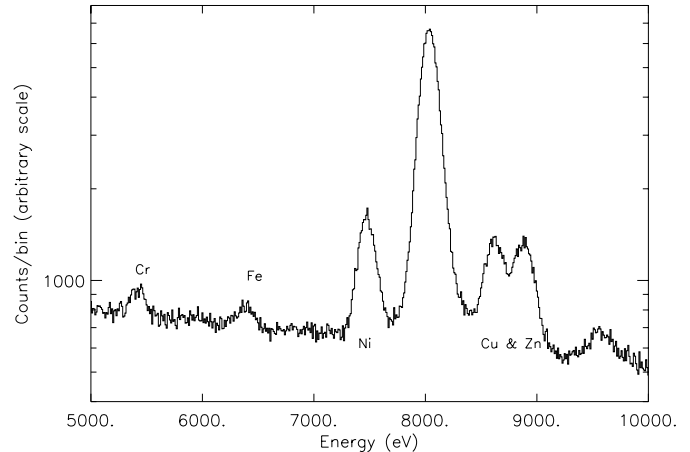
Fig. 5. Spectrum from the PN camera around the region of the Cu K 8.05 keV emission line, showing fluorescent emission from other camera body materials.
