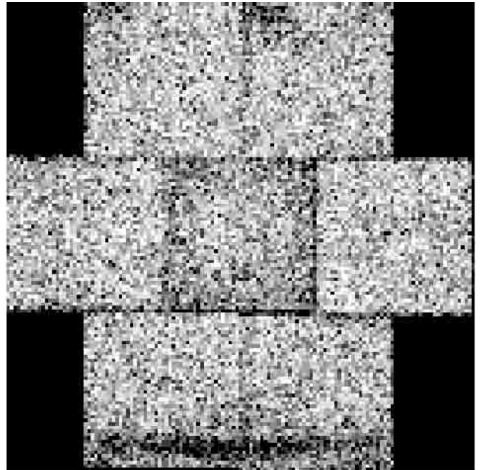
Fig. 2. Image from the MOS camera formed in the energy band of Al K fluorescent emission. Gaps between the chips are barely visible but some shadowing features at the top and bottom are evident (due to cut outs in the camera body for internal calibration sources). The rim areas of the central CCD are significantly dimmer than those of surrounding chips, because the CCD lies slightly below the others, and there is thus shadowing of any emission from the camera body above the focal plane.
