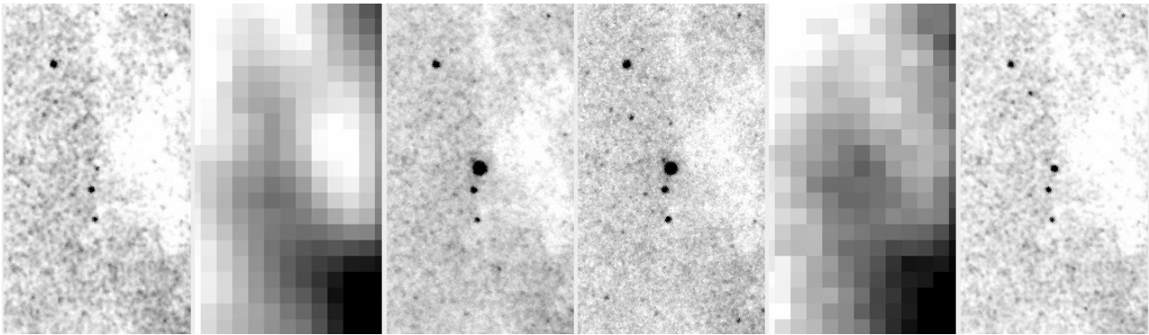
Fig. 1. Images of M31N 2004-11f: from the left to the right HST-ACS ( F435W ) 2004-01-23, Wendelstein (R) 04-10-25, HST-ACS ( FR423N ) 2004-11-02, HST-ACS ( FR388N ) 2004-11-08, Wendelstein (R) 04-11-09, HST-ACS ( F435W ) 2004-11-22. The different bands are given in brackets. The angular scale of each image is 6'' \times 10.5'' . Note that already in the first image the pre-nova is clearly identified. Due to the lower resolution the faint source is not visible in the second image taken on Wendelstein previous to the nova outburst. After the outburst the nova is also visible in the fifth image from Wendelstein.
