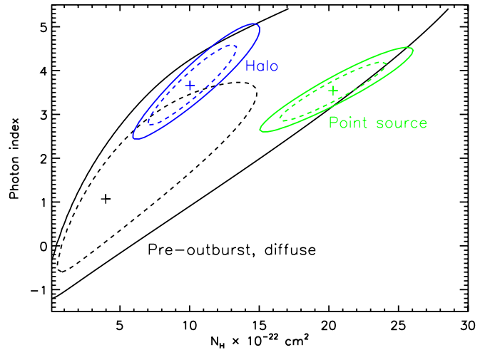
Figure 10. Confidence contours (68% and 90%) in the N_{\text{H}}-\Gamma plane for the PL fit to the halo (blue), point source (green), and the pre-outburst diffuse emission (black) spectra. The contours are obtained with the PL normalization fitted at each point of the grid. The best-fit parameter values are shown by crosses.
