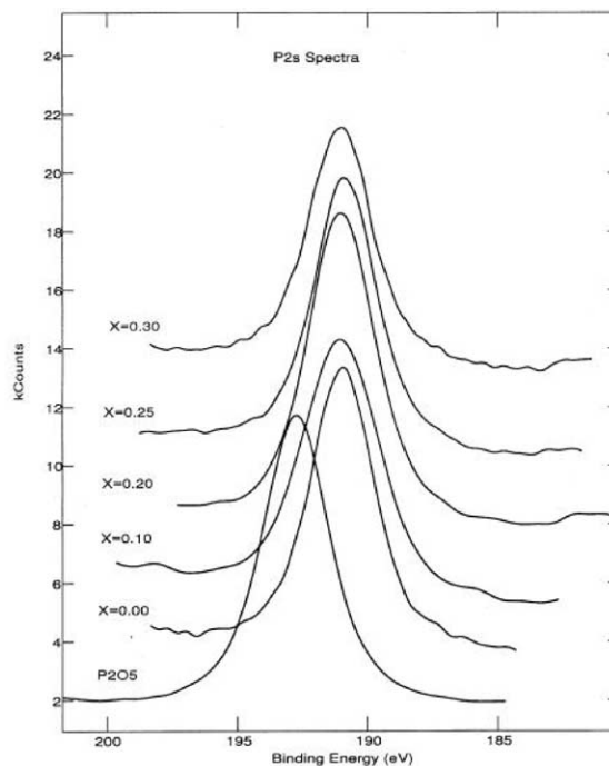
Fig. 7. High-resolution P 2s spectra for the \text{Fe}_2\text{O}_3 vanadium phosphate glasses and \text{P}_2\text{O}_5 powder.
