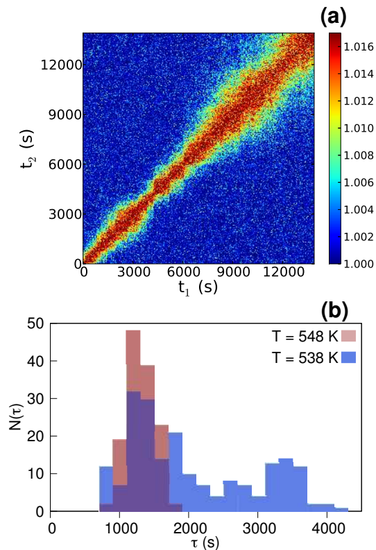
FIG. 3. (a) Measured TCF at T = 538 K after step-cooling from 548 K. The overall broadening of the intensity profile reflects a slowing down of the microscopic dynamics corresponding to physical aging. (b) Distribution of \tau during stationary dynamics ( T = 548 K) and heterogeneous aging dynamics ( T = 538 K).
