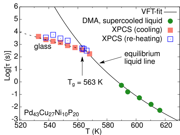
FIG. 1. Structural relaxation times measured with DMA (filled circles) and XPCS during slow cooling from the supercooled liquid (filled squares) and subsequent re-heating from the partially annealed glass (open squares). The solid line is a fit of the equilibrium data to the VFT equation. The dashed line is an Arrhenius fit to the XPCS cooling data in the glass.
