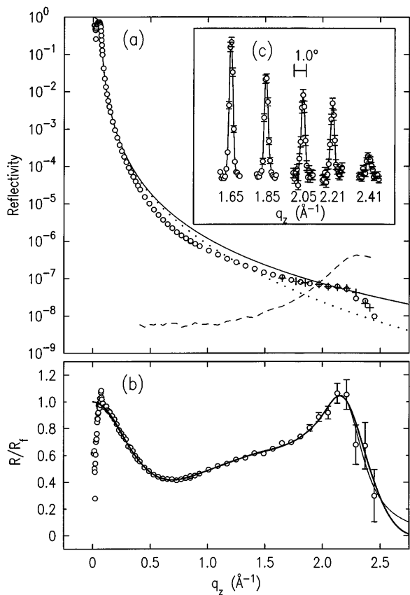
FIG. 1. (a) X-ray reflectivity of the free surface of liquid mercury at room temperature under \text{H}_2 (○); (+) indicates values calculated from the transverse 2\theta scans in (c). In addition, the Fresnel reflectivity R_f for an ideally flat surface (—), the reflectivity of an interface with a roughness given by the convolution of the Hg atomic form factor and a Gaussian of 0.8 \text{ \AA} width (⋯), and the background intensity (---) are shown. (b) Experimental data (○) and two fits (—) of the ratio R/R_f . (c) Selected 2\theta scans across the reflected beam at various q_z \geq 1.5 \text{ \AA}^{-1} ( -0.8 \leq 2\theta \leq 0.8 , background subtracted).
