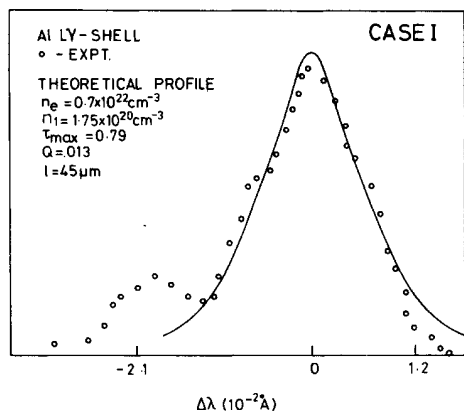
FIG. 9. A fit of the Al III Ly surface plasma emission to a theoretical profile.
