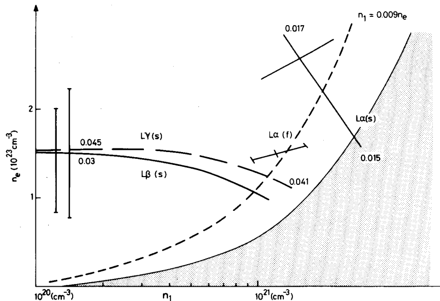
FIG. 13. The lines of best fit in the n_e , n_1 parameter space for the silicon Lyman emission lines from the core. The fits of the L\alpha line using standard L\alpha(s) and full L\alpha(f) calculations of the optically thin profiles are shown. The shaded area is the forbidden region.
