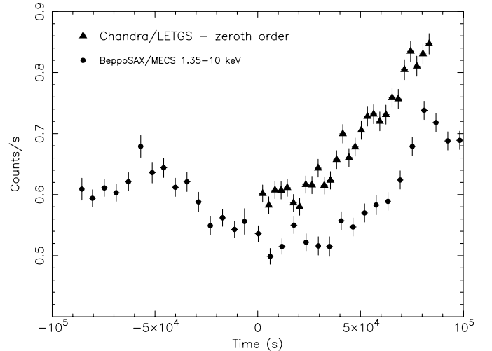
Fig. 4. Light curve of NGC 5548 for the zeroth spectral order of the LETGS and the BeppoSAX MECS data. Bin size of the LETGS data is 3000 s, the MECS data have been averaged per satellite orbit. Zero point is the start time of the LETGS data.
