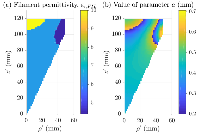
Fig. 7. (a) Using the permittivity profile of Fig. 2(a) and the model of Fig. 6(c), the filament to be used at each point of the radiator is determined. (b) Knowing which filament will be used, the value of parameter a is determined using the appropriate homogenization curve in Fig. 6(b).
