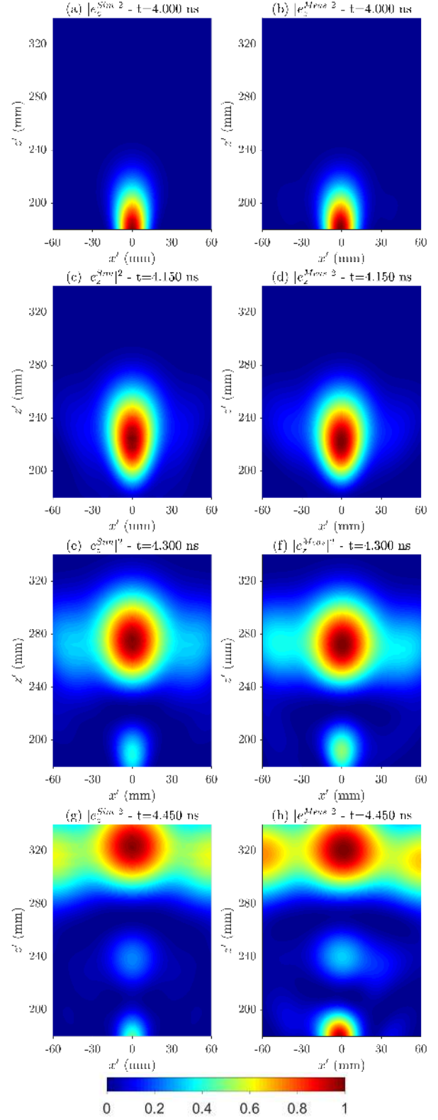
Fig. 16. The intensity of the longitudinal ( z' -directed) electric field in the region over the radiator as a function of space and time when excited with a uniform spectrum pulse (7.5 – 12.5 GHz): using (a) simulation and (b) measurement results at 4 ns, (c) simulation and (d) measurement results at 4.15 ns, (e) simulation and (f) measurement results at 4.3 ns, (g) simulation and (h) measurement results at 4.45 ns.
