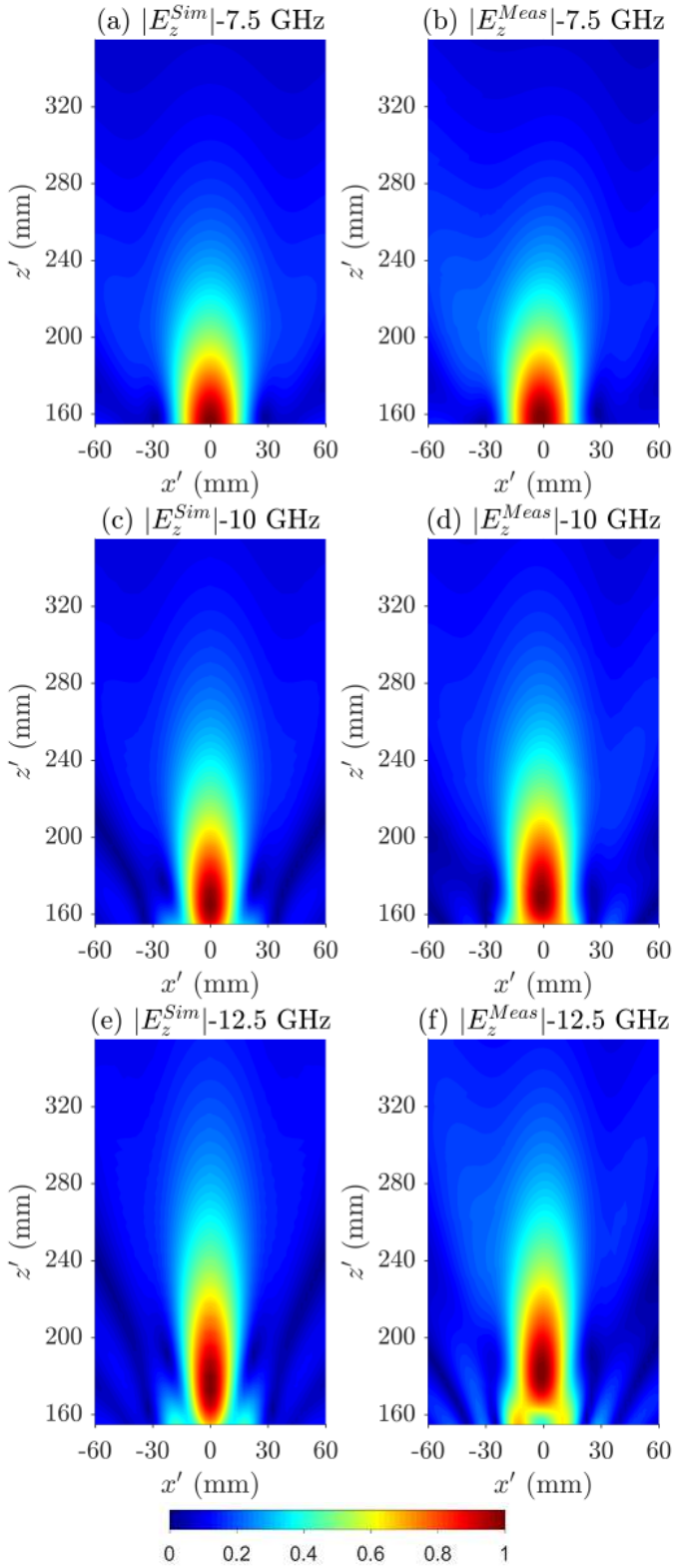
Fig. 15. The longitudinal ( z' -directed) electric field in the region over the radiator: (a) simulation and (b) measurement results at 7.5 GHz, (c) simulation and (d) measurement results at 10 GHz, (e) simulation and (f) measurement results at 12.5 GHz.
