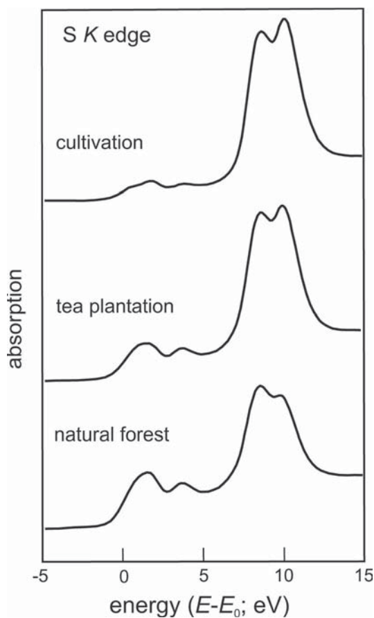
FIG. 21. Sulfur K -edge XANES spectra for humic substances extracted from clay (<2 μm) separates of soils from Wushush, southwestern highlands of Ethiopia, showing progressive loss of reduced and intermediate-oxidation-state S with more extensive cultivation. The photoelectron energy is relative to the absorption threshold (after Solomon et al. 2003).
