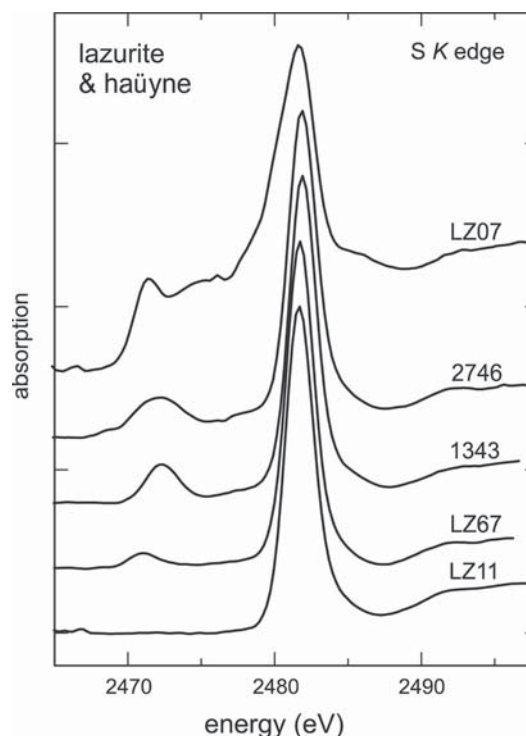
FIG. 18. Sulfur K -edge XANES spectra for synthetic h a y ne (LZ11) and lazurite from Afghanistan (2746), Baffin Island (1343) and hydrothermal-pressure (LZ67) synthesis. Note that the spectrum of colorless h a y ne contains a single edge-peak for sulfate, whereas royal-blue lazurite (2746, 1343 and LZ67) contains both reduced S and sulfate species, and LZ07 contains thiosulfate and sulfate species (after Fleet et al. 2005b).
