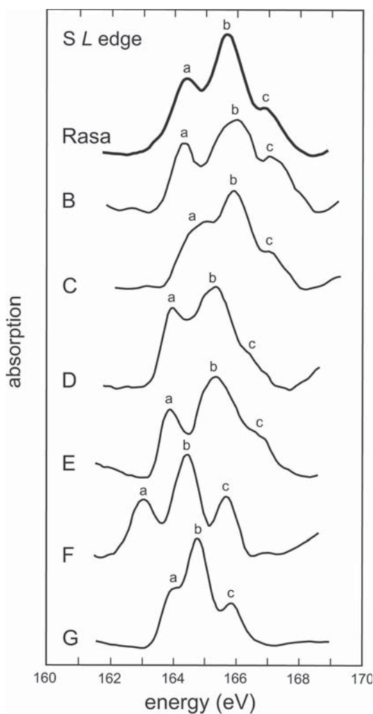
FIG. 19. Sulfur L -edge XANES spectra for a standard coal from Rasa (Croatia) and reference organic S compounds, including: (B) 1,2-benzodiphenylene sulfide, (C) thioxanthen-9-one, (D) phenyl disulfide, (E) poly(phenylene sulfide), (F) DL-cystine and (G) S-methyl-L-cysteine. The best match for the Rasa coal was obtained with 40% thiophenic S (B), 30% thioxanthone (C) and 30% aryl disulfide (D) (after Kasrai et al. 1996b).
