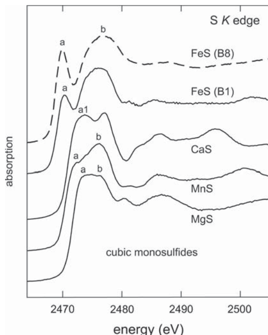
FIG. 10. Sulfur K -edge XANES spectra for rocksalt (B1) structure FeS, oldhamite (CaS), alabandite (MnS) and niningerite (MgS), compared with spectrum for troilite (FeS); spectra were recorded by fluorescence yield (after Farrell et al. 2002).
