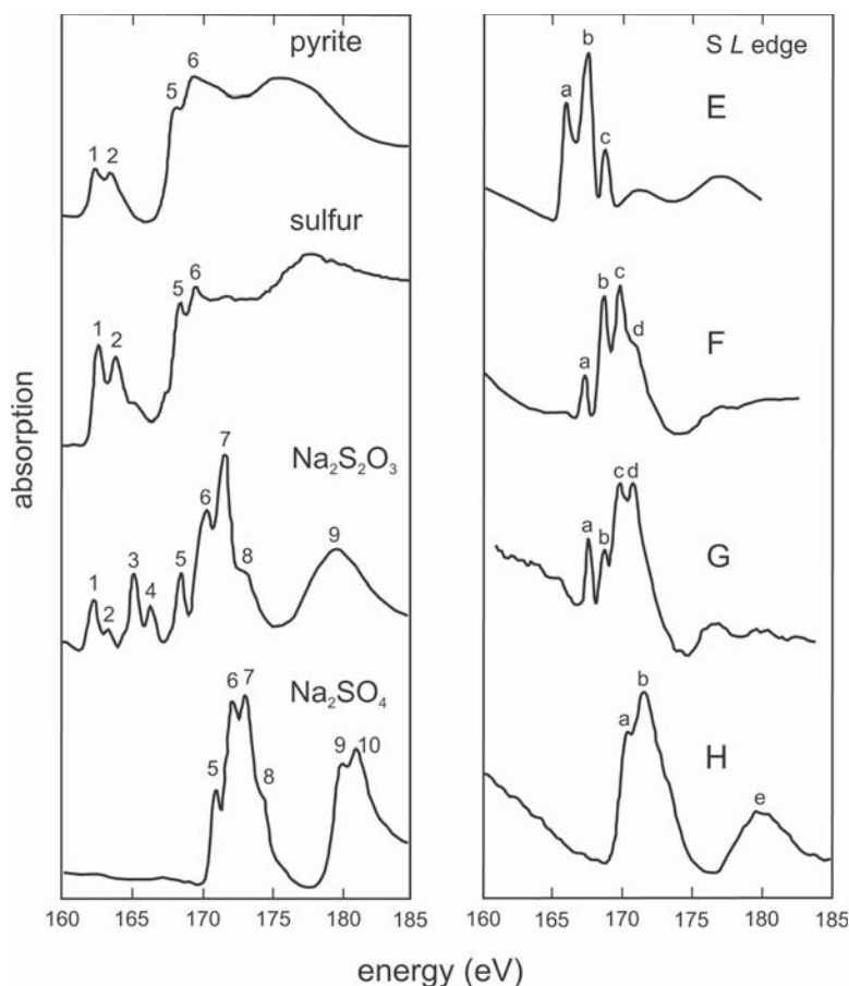
FIG. 3. Sulfur L -edge XANES spectra for some reference compounds, including pyrite, native S, sodium thiosulfate, sodium sulfate, (E) DL-methionine sulfoxide, (F) dibenzothiothiophene sulfone, (G) poly(1,4-phenylene ether-sulfone) and (H) sodium anthraquinone-2-sulfonic acid (after Kasrai et al. 1996b).
