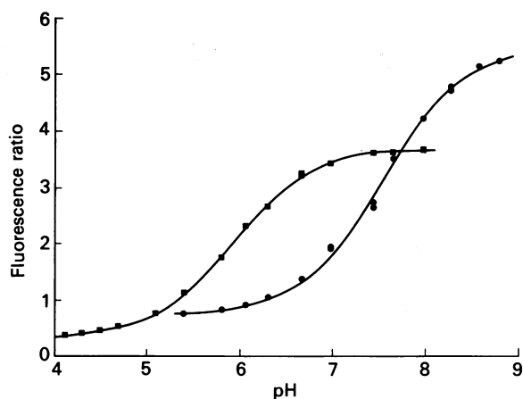
Fig. 1. pH-dependence of the fluorescence ratio of sodium fluorescein and of FLPE in phospholipid vesicles
