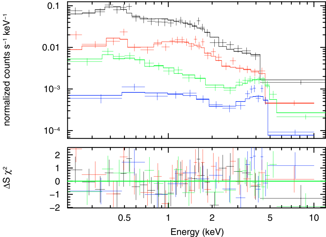
Fig. 3. The EPIC spectra of both observations plotted in comparison to a model consisting of a continuum power law and a relativistically blurred X-ray ionised reflection component that originates in an accretion disk near to a supermassive black hole. Both components are seen through a warm absorber (Table 4, fit 23). The ionisation parameter of the warm absorber and the normalization of the continuum components were free to vary. The deep minimum state is dominated by the reflection component while the power law component vanishes.
