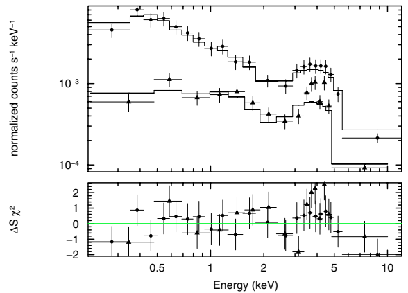
Fig. 2. The two (MOS and pn) EPIC spectra of the deep minimum state of PG 2112+059 are shown in comparison to a spectral model that consists of a continuum power law behind two layers of absorbing material (Table 4, fit 10). The upper spectrum was taken with the EPIC pn camera and the lower one with the MOS cameras. The model is not able to describe the spectra well at energies above 3 keV as there are systematic residua visible in the lower panel.
