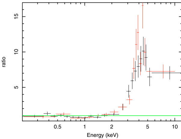
Fig. 1. The ratio between the EPIC data of the deep minimum state of PG 2112+059 and a hypothetical canonical power law spectra with a photon index of \Gamma = 2 behind Galactic absorption is shown. The pn data points are given in black and the MOS data points are printed in red, respectively.
