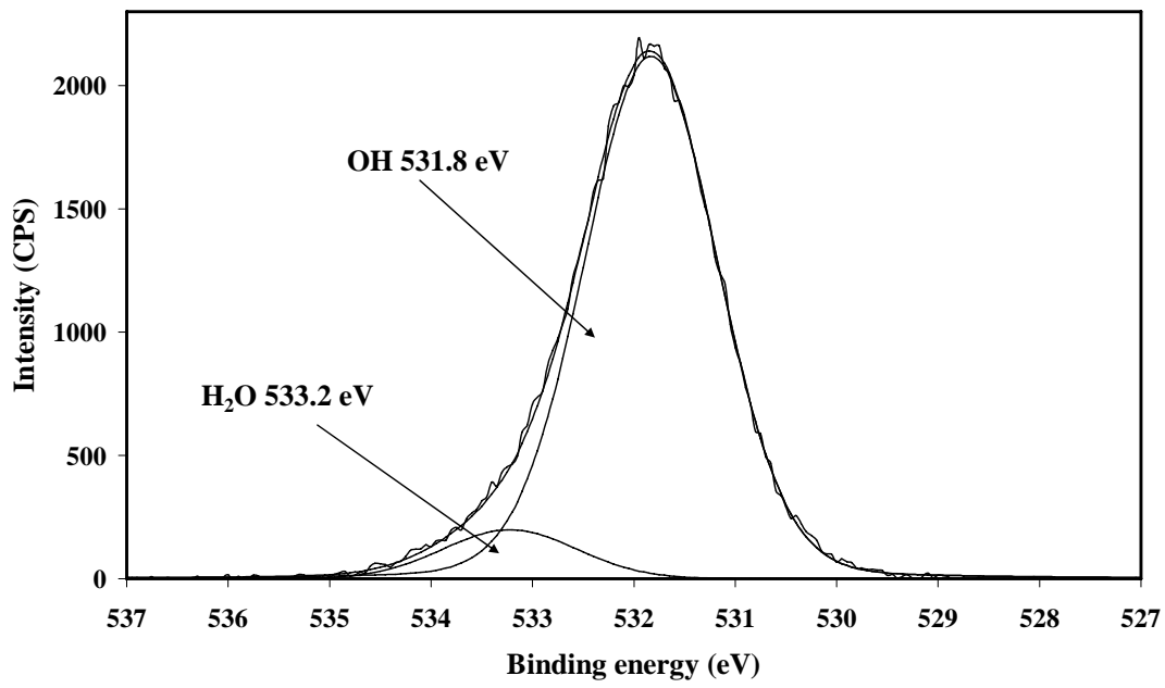
Fig 1b O 1s gibbsite
