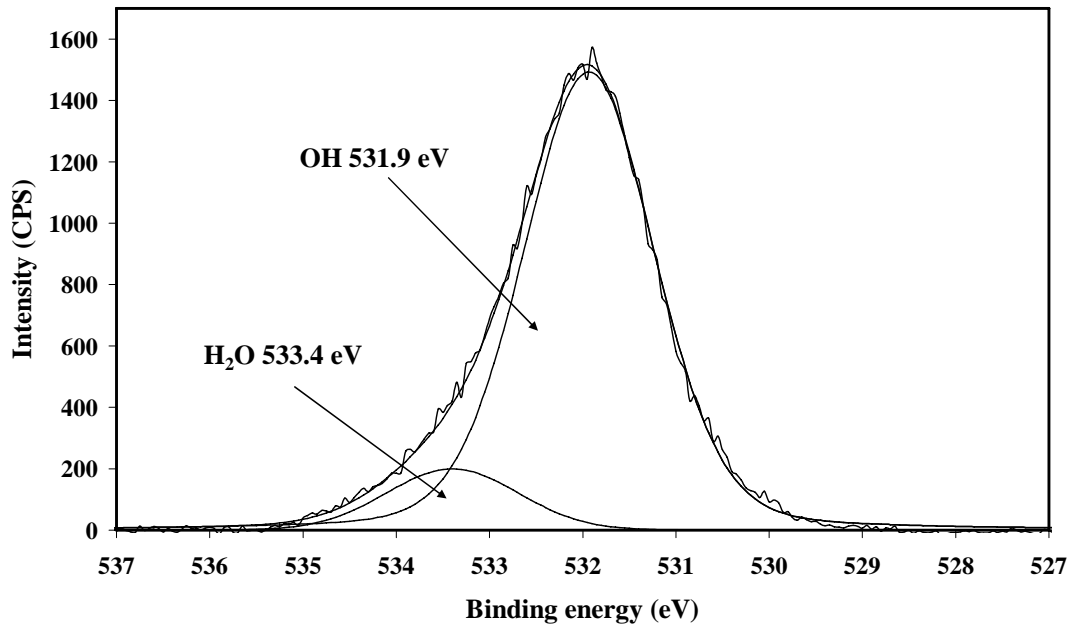
Fig 1c O 1s bayerite
