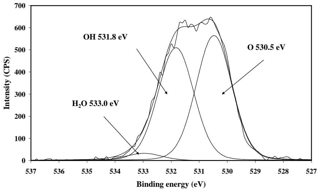
Fig. 1d O 1s boehmite
