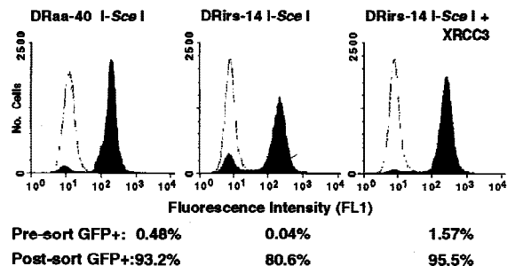
Figure 3. Green fluorescence is stably expressed after I-Sce I expression. Wild-type DRaa-40 cells and XRCC3-deficient DRirs-14 cells were electroporated with the I-Sce I expression vector or both the I-Sce I and XRCC3 expression vectors, sorted on the basis of green fluorescence, and then reanalyzed by flow cytometry. Percent GFP+ cells before sorting (unshaded peak) and after sorting (shaded peaks) are indicated. Not shown is the DRaa-40 cell line transfected with both the I-Sce I and XRCC3 expression vectors, in which the presorted population was 0.66% GFP+ and the post-sorted population was 93.5% GFP+. Also not shown are the lacZ -transfected cells that were not sorted; 0.01% GFP+ for DRaa-40 and <0.01% GFP+ for DRirs-14. (The frequency of GFP+ cells is lower in this experiment than the one shown in Fig. 2, because only 20 \mu\text{g} of each of the expression vectors was electroporated.)
