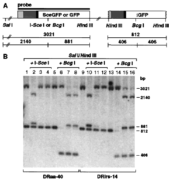
Figure 4. Green fluorescence is a measure of STGC. (A) Map of the parental or recombined DR-GFP substrate containing SceGFP or GFP , respectively. Sizes of expected fragments are indicated in base pairs. (B) Southern blot analysis of sorted cell lines. Genomic DNA was digested with the indicated endonucleases. (Lanes 1,2,5,6) Untransfected wild-type cell line DRaa-40; (lanes 3,7) GFP+ DRaa-40 cells from transfection of the I-Sce I expression vector; (lanes 4,8) GFP+ DRaa-40 cells from cotransfection of the I-Sce I and XRCC3 expression vectors; (lanes 9,10,13,14) untransfected mutant cell line DRirs-14; (lanes 11,15) GFP+ DRirs-14 cells from transfection of the I-Sce I expression vector; (lanes 12,16) GFP+ DRirs-14 cells from cotransfection of the I-Sce I and XRCC3 expression vectors. The residual 3021-bp band after BcgI digestion in lanes 7,8,15, and 16 is likely due to GFP-negative cells in the population (see Fig. 3).
