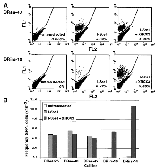
Figure 2. The irs1SF cell line is defective for DSB-induced homologous recombination because of XRCC3 deficiency. Wild-type (DRaa) and XRCC3-deficient (DRirs) cell lines were electroporated with each of the indicated expression vectors ( 100 \mu\text{g} of the I-Sce I vector; 20 \mu\text{g} of the XRCC3 vector), and 5 \times 10^4 cells were analyzed by flow cytometry. (A) Two-color fluorescence analysis for cell lines DRaa-40 and DRirs-10. The percentage of green fluorescent cells falling above the diagonal for each transfection are indicated. (FL1) Green fluorescence; (FL2) orange fluorescence. (B) Summary of results from several cell lines.
