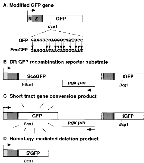
Figure 1. GFP expression plasmids. (A) Modified GFP gene. The modified GFP gene encodes the EGFP protein fused to a nuclear localization signal (N) and zinc finger domain (Z). It is expressed from a hCMV enhancer/chicken \beta -actin promoter (arrow) on a spliced message (not shown). GFP is modified to SceGFP so as to contain an I-Sce I site and in-frame termination codons (underline). (B) DR-GFP recombination substrate. Downstream of the SceGFP gene is iGFP , a 5' and 3'-truncated GFP gene. (C) (STGC) product. In a STGC, a DSB at the I-Sce I site is repaired from the iGFP gene on the same chromatid or sister chromatid, to result in a functional GFP gene. (D) Homology-mediated deletion product.
