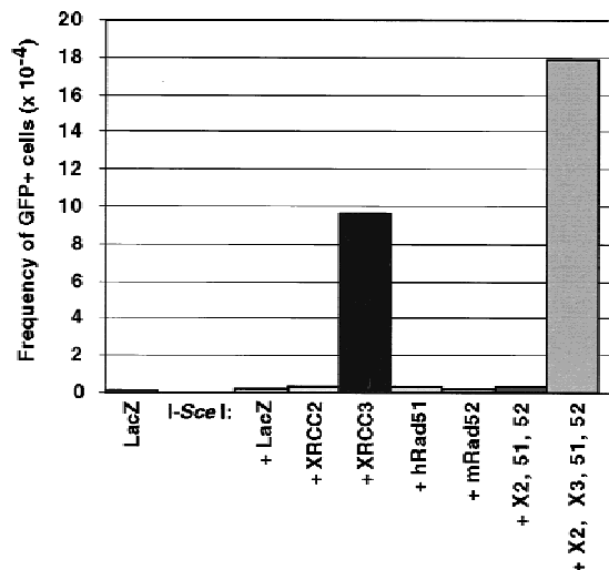
Figure 5. DSB-induced recombination is restored in the irs1SF cell line by transient expression of XRCC3 but not other recombination proteins. The DRirs-14 cell line was electroporated with each of the indicated expression vectors (20 \mu g). The total amount of DNA electroporated was maintained at a constant level by the addition of pCMV- lacZ . A total of 5 \times 10^5 cells were analyzed by flow cytometry. (hRad51 or 51) Human Rad51; (mRad52 or 52) mouse Rad52; (X2) XRCC2; (X3) XRCC3.
