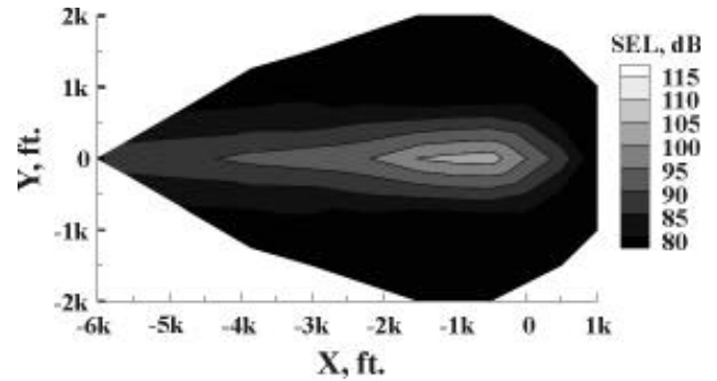
Figure 13. SEL contour for a typical takeoff condition.
