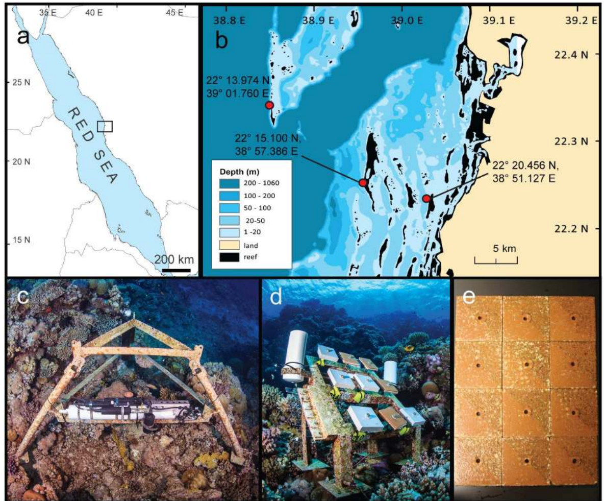
Fig 1. Map of study area and set up of coral reef monitoring sites in the central Red Sea. (a) The study area is located in the central Red Sea, (b) with three study sites (red markers) across the shelf. (c) Loggers (CTDs and ADCPs) for continuous data collection were moored to aluminum tripods fixed to the reef at 7–9 m depth. (d) Sediment traps and tiles were mounted on an aluminum frame fixed to the reef. (e) Sampled tiles after scraping off half of the biofilm for 16S rRNA gene amplification. Image credits: (a, b) Maha Khalil; (c, d) Tane Sinclair Taylor; (e) Stephan G. Kremb.
