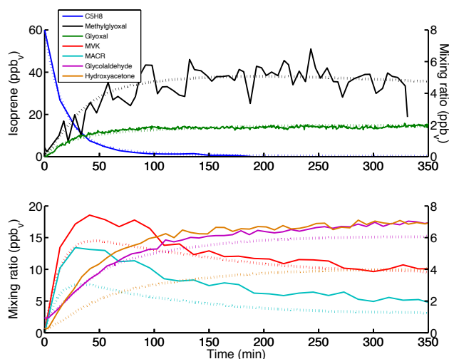
Fig. 3. Model and measurement comparison for high-NO x isoprene oxidation (Exp. 7) using the modified MCM model. The glycolaldehyde to glyoxal yield was set to 29%, and first generation yields of glyoxal (2.6%), methylglyoxal (2.7%), hydroxyacetone (2.6%), and glycolaldehyde (2.7%) were included in this model run. Glyoxal production from C5 hydroxycarbonyls was attenuated to 1/6 of the MCM v. 3.2 values.
