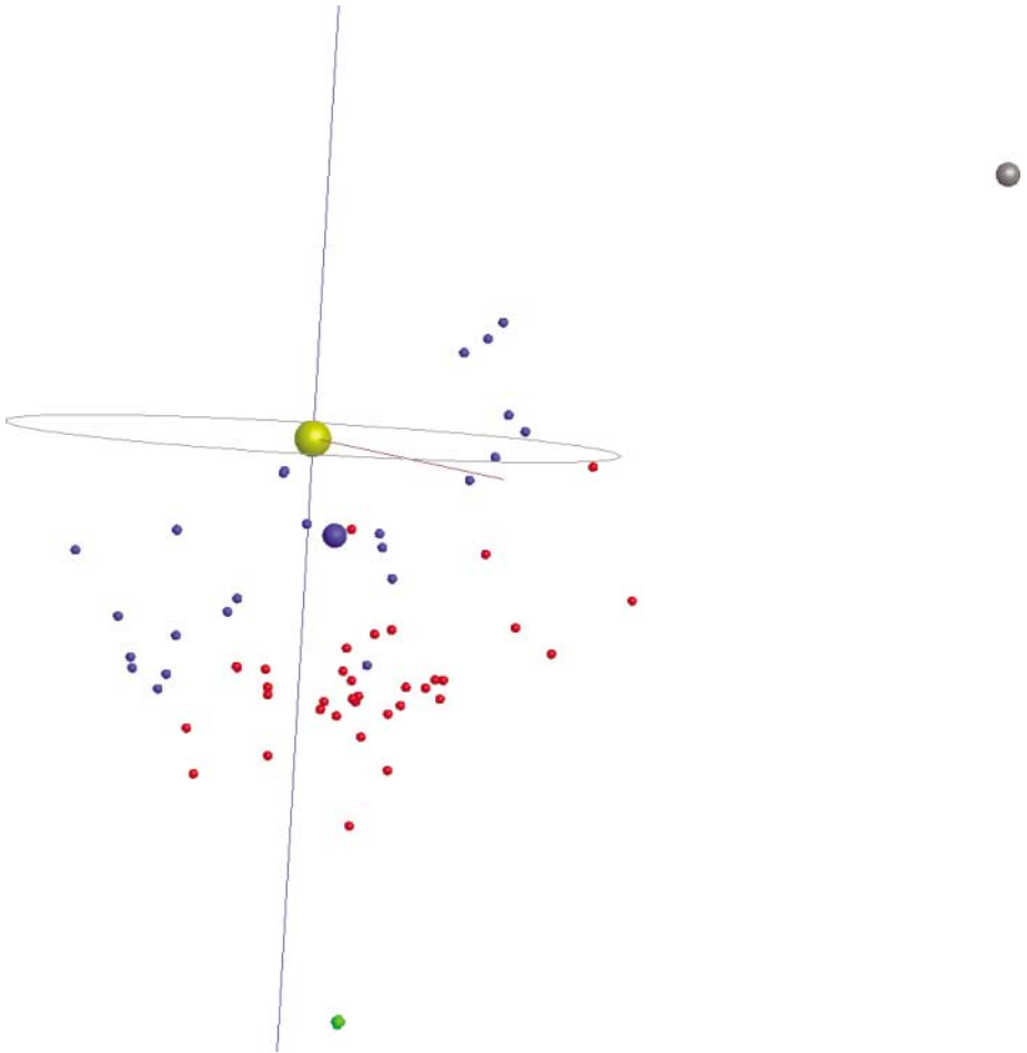
Figure 1 Widespread distribution of members of the \beta Pic and Tucana/Horologium Associations contrasted with the more distant and much more spatially concentrated Pleiades ( gray dot ) and \eta Cha ( green dot ) clusters, shown approximately to scale. The oval represents a distance of 50 pc from the Sun ( yellow ball ). Note the concentration to deep in the Southern Hemisphere. The large blue dot is \beta Pic. Blue dots represent \beta Pic members, and red dots represent Tucana/Horologium Association members.
